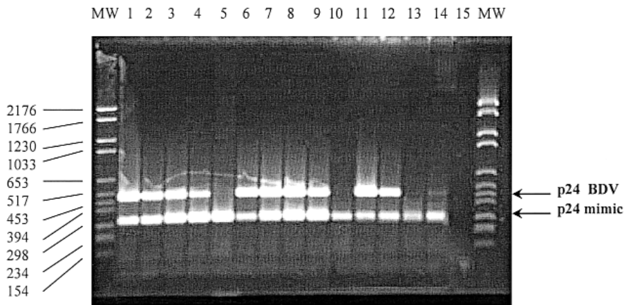
Figure 3. RT-PCR test with both BDV and mimic RNA in biological samples (2% agarose gel). MW: molecular weight; lanes 1 to 4: decreased dilutions of BDV infected VERO cells; lane 5: BDV infected VERO cells; lanes 6 to 9: decreased dilutions of BDV infected VERO cells in blood; lane 10: non infected VERO cells in blood; lanes 11 to 14: decreased dilutions of BDV infected VERO cells in brain; lane 15: non infected VERO cells in brain.
