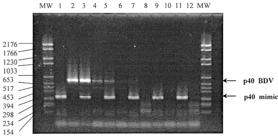
Figure 2. RT-PCR with various purified BDV RNA dilutions and constant p40 mimic RNA concentration (2.5 fg) on a 2% agarose gel. MW: molecular weight; lane 1: p40 RNA mimic; lane 2: 0.1 ng of purified BDV RNA; lane 3: p40 RNA mimic and 0.1 ng of purified BDV RNA; lane 4: 100 pg of purified BDV RNA ; lane 5: p40 RNA mimic and 100 pg of purified BDV RNA; lane 6: 10 pg of purified BDV RNA; lane 7: p40 RNA mimic and 10 pg of purified BDV RNA; lane 8: 1 pg of purified BDV RNA; lane 9: : p40 RNA mimic and 1 pg of purified BDV RNA; lane 10: 0.1 pg of purified BDV RNA; lane 11: : p40 RNA mimic and 0.1 pg of purified BDV RNA; lane 12: negative control (without any RNA template).
