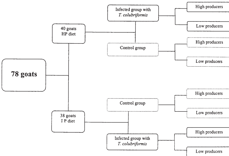
Figure 1. Protocol design.
