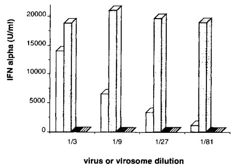
Fig 2. Induction of IFN- \alpha by TGEV ( \square ), concentrated TGEV ( \blacksquare ) and virosomes (OG ( \square ) and NaDOC/NP40 ( \boxtimes )). PBMC were induced to produce IFN- \alpha in an overnight incubation with the different viral preparations. Concentrated TGEV and virosomes were tested using roughly equivalent amounts of viral material. IFN- \alpha levels in the supernatant culture was assayed by the specific immunoassay.
