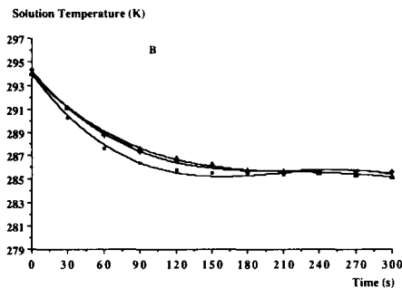
Fig 6. Influence of the pressure on the temperature changes in the nebulization solution when the feed pipe for compressed air was immersed in a water bath with average temperatures 276.9 \pm 0.4 (A) and 311 \pm 0.7 K (B).
