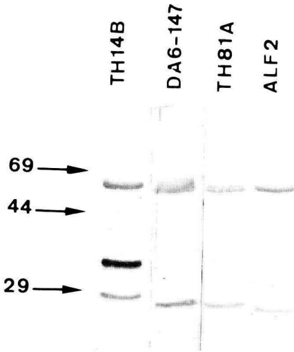
Fig 1. DA6-147 reactivity on western blotting of surface molecules previously recognized by mAbs TH14B, DA6-147, TH81A and ALF-2 (anti-feline lymphocytes, used as negative control). Marker protein relative mass (kDa) is indicated at the side. Fainter entities at 25 and 56 kDa represent heavy and light immunoglobulin chains.
