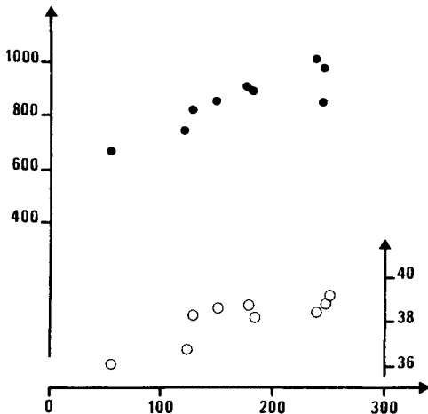
Fig. 3. — Relationship between heat production, rectal temperature and colostrum intake in piglets kept at 18 °C during the first 24 h after birth (according to Noblet and Le Dividich, 1981).
