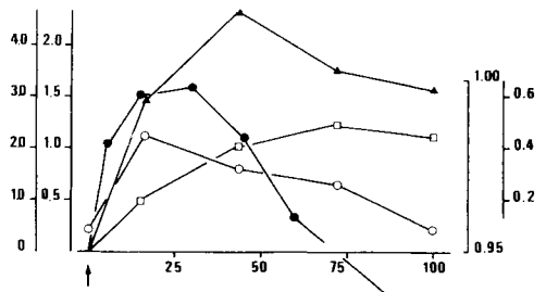
Fig. 4. — Effect of colostrum intake on RQ (○) and increment in VO_2 (▲), RT (□) and blood glucose (●) in piglets kept at 18 °C (according to Noblet and Le Dividich, 1982).
