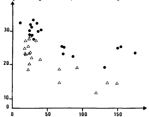
Fig. 2. — Oxygen consumption of neonatal unfed pigs kept in cold (●, 18 °C) and warm (△, 31 °C) conditions in the immediate period following birth (according to Noblet and Le Dividich, 1981).
