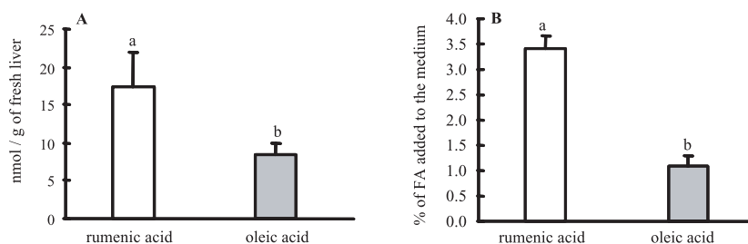
Figure 1. Uptake of ruminic and oleic acids by bovine liver slices. Liver slices from bovine animals were incubated in a medium containing a FA mixture (0.75 mM) and [ 1-^{14}\text{C} ] ruminic acid or [ 1-^{14}\text{C} ] oleic acid for 17 h. The FA uptake was calculated as the sum of FA converted into \text{CO}_2 , into ASP, and incorporated into total cellular lipids. The values are expressed in nmol per g fresh liver (A) or as % FA added in the medium (B). The data are means \pm SEM of 5 animals per group for ruminic acid uptake and 3 animals per group for oleic acid uptake. Mean values with different superscripts were significantly different ( a,b P < 0.01 ).
