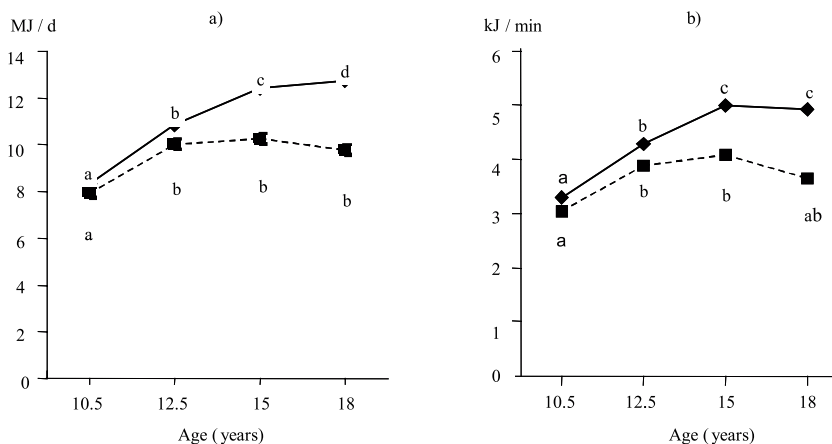
Figure 3. Changes in daily energy expenditure (a) and sleeping energy expenditure (b) in boys (—) and girls (- - -) with a standardised activity programme in the whole-body calorimeters, between 10 and 18 years of age (values with different superscripts are significantly different between age groups and genders).
