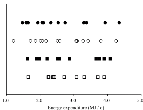
Figure 7. Inter-individual variability in energy expenditure associated with physical activities in obese ( \square ) or post-obese ( \blacksquare ) boys, and in obese ( \circ ) or post-obese ( \bullet ) girls in free-living conditions (mean values over a week).
