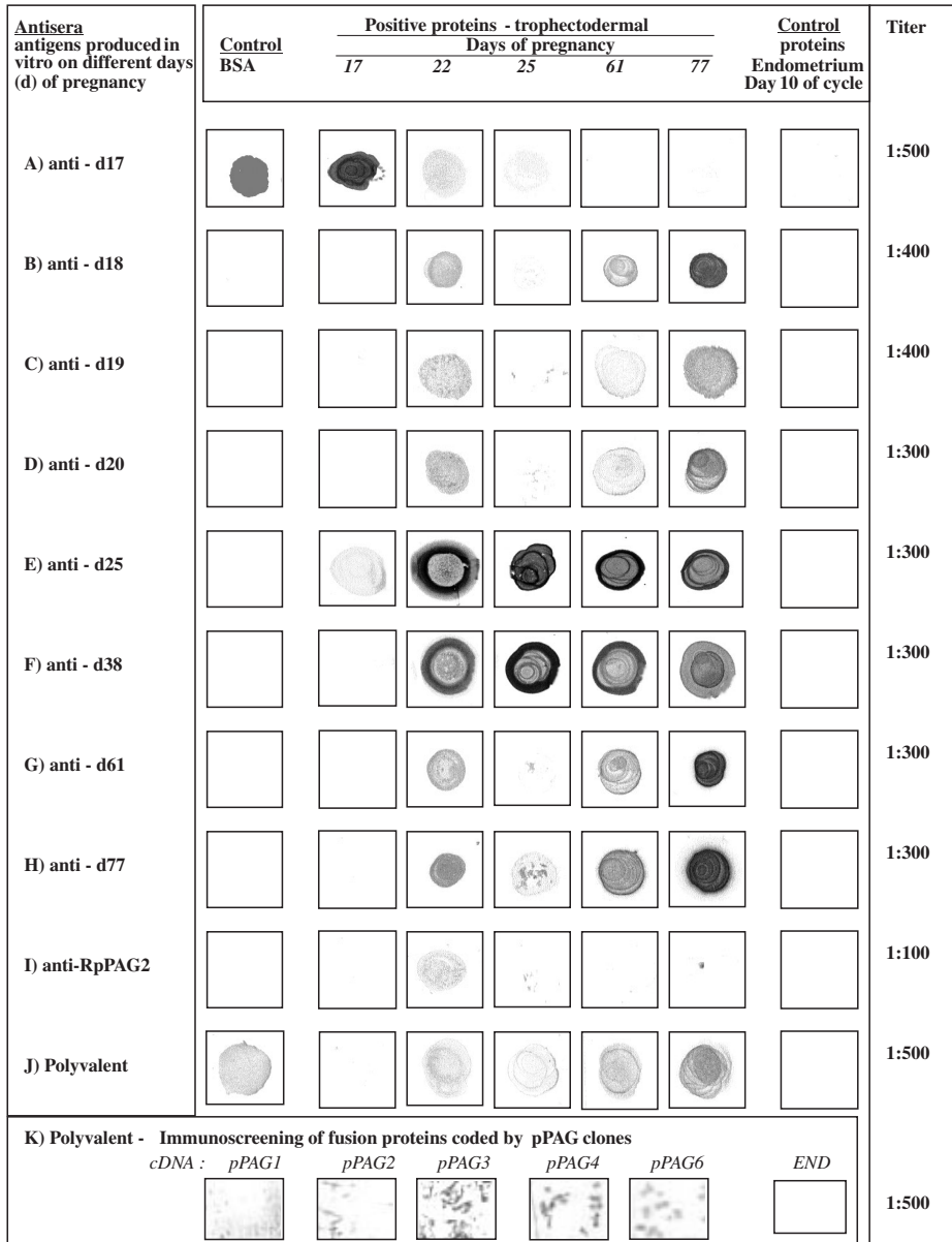
Figure 4. The cross-reactions of adsorbed polyclonal antisera (A–J, in titers from 1:100 up to 1:500) with different ( 5 \mu\text{g}\cdot\text{sample}^{-1} ) porcine native trophoctodermal proteins produced in vitro (from Days 17, 22, 25, 61 and 77) or control proteins (BSA and END10) analysed by Western dot-blotting. Unspecific bounding of each antiserum has been removed by adsorption with endometrial tissues or endometrial proteins produced in vitro. (K) Specificity of purified polyvalent anti-pPAG serum identified by immunoscreening of various pPAG cDNA clones isolated from a porcine trophoblastic cDNA library in contrast to the lack of cross-reactions to endometrial cDNA library.
