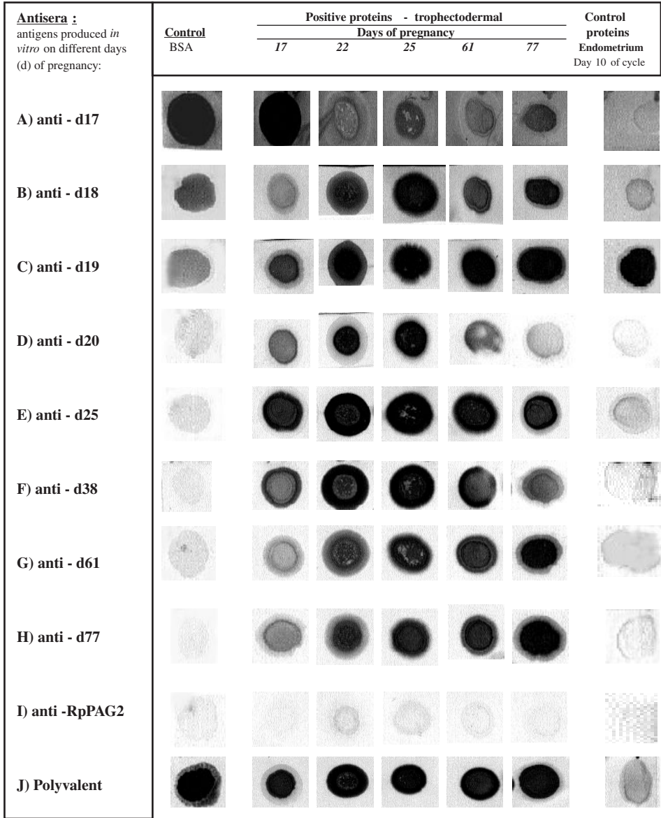
Figure 3. Western dot-blot analysis of the pPAG proteins produced in vitro ( 5 \mu\text{g}\cdot\text{sample}^{-1} ) or control proteins (BSA and END10) with crude polyclonal antisera (in titer 1:300) obtained from rabbits immunised against different porcine antigens: native trophoctodermal proteins (A–H), or recombinant pPAG2 protein (I) and mixed “diagnostic” polyvalent antisera (J).
