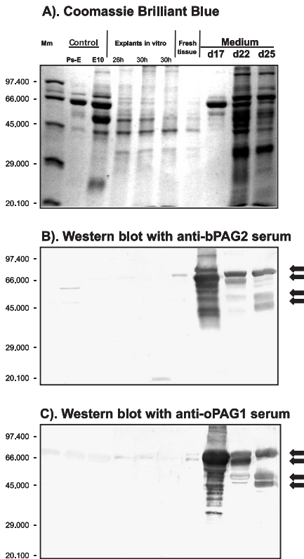
Figure 1. The effectiveness of the pPAG protein isolation monitored by cross-species Western analyses. Trophoctodermal proteins isolated from fresh (Day 21 of pregnancy) or cultured tissues (Days 20 and 21) were compared to proteins released in vitro into the media by cultured (8 h) different explants of the trophoblast (Days 17, 22 and 25 of pregnancy) or endometrium of cyclic (E10) and pseudopregnant gilts (Ps-E). (A) Stained porcine proteins ( 10 \mu\text{g}\cdot\text{sample}^{-1} ) separated in 12.5% gel. Molecular markers (Mm) are shown on the left. Duplicates of proteins transferred onto the membranes were exposed to (B) polyclonal antisera raised against bPAG2, or (C) to polyclonal antisera raised against oPAG1. The arrows on the right indicate immunoreactive bands of the pPAG-like proteins detected by antisera produced against single purified ruminant PAG proteins.
