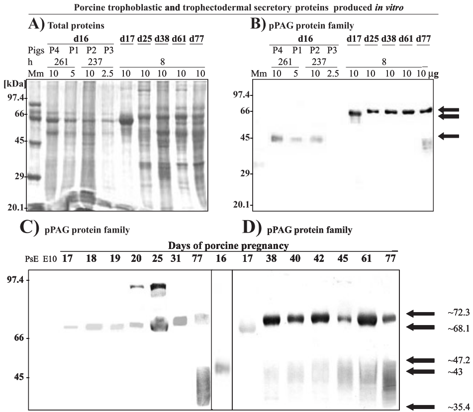
Figure 8. Production efficiency and immunodetection sensitivity of total proteins (2.5–10 µg-sample -1 ) secreted in vitro by trophoblastic explants (237–261 h) recovered from pigs on day 16 (P1–P4) and by trophectodermal explants (8 h) recovered on various days (d17–d77) of pregnancy. (A) SDS-PAGE of total chorionic proteins stained by CBB dye. (B–D) Western blot of secretory pPAG proteins during early embryonic and foetal development throughout porcine pregnancy detected by polyvalent “diagnostic” anti-pPAG serum. Arrows on the right indicate apparent M r (kDa) of the pPAG proteins.
