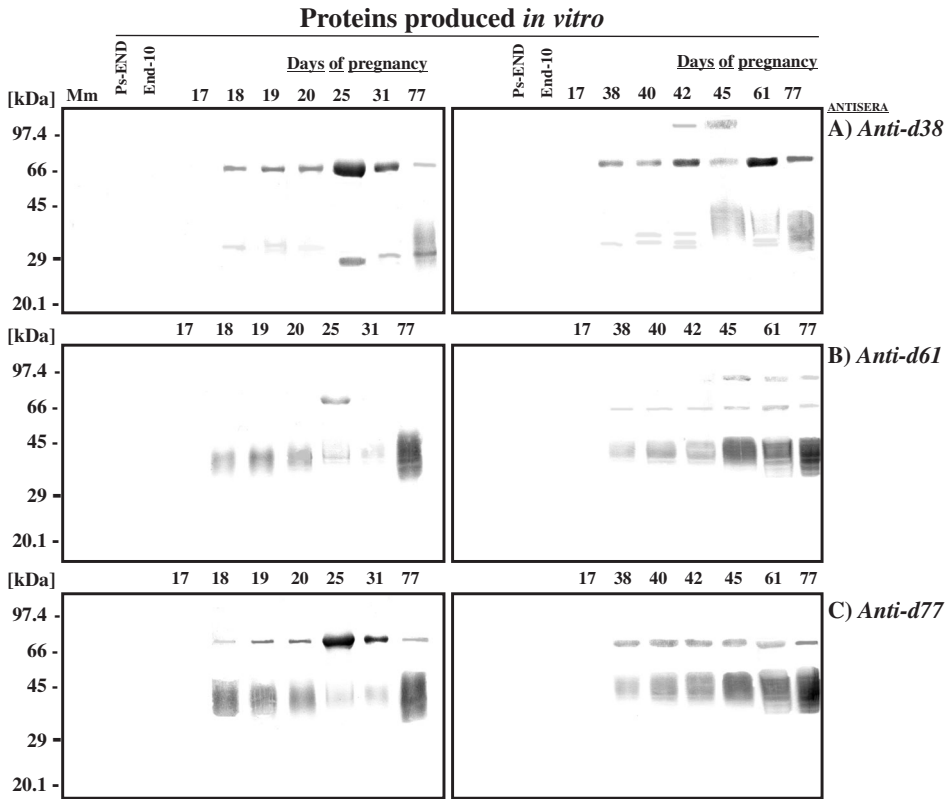
Figure 7. The heterogeneous products of the pPAG gene family examined during various stages of embryonic and foetal developments throughout pregnancy. (A–C) Western blot (1D-SDS-PAGE) of secretory proteins produced in vitro ( 10 \mu\text{g}\cdot\text{sample}^{-1} ) by trophoblast explants (Days 17–77) and control endometrial explants of cyclic (End10) and pseudopregnant (Ps-END) gilts. Membranes were blotted with different purified antisera raised against various porcine immunogens (anti-d38, anti-d61 and anti-d77 sera). Molecular markers (Mm) are on the left.
