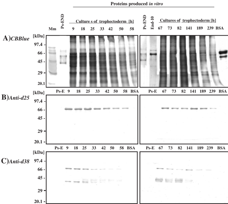
Figure 5. The heterogeneous products of the pPAG gene family examined during long-term studies of trophoctodermal explants harvested on day 24 of pregnancy and cultured for 239 h. (A) CBB-stained proteins (1D-SDS-PAGE) separated in 12.5% gel. Secretory proteins produced in vitro ( 10 \mu\text{g}\cdot\text{sample}^{-1} ) by trophoctodermal explants during 9–239 h and negative control proteins: endometrial explants of cyclic (End10) and pseudopregnant (Ps-END) gilts or BSA (non-specific for pregnancy) were compared. (B–C) Duplicates of proteins were transferred onto membranes that were blotted with different antisera raised against porcine antigens (anti-d25 and anti-d38). Molecular markers (Mm) are on the left.
