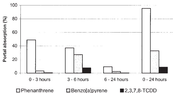
Figure 4. Portal absorption rate of ^{14}\text{C} after ingestion by the growing pig of 1000 mL milk spiked with ^{14}\text{C} phenanthrene, ^{14}\text{C} benzo[a]pyrene or ^{14}\text{C} 2,3,7,8-TCDD (mean value, n = 2 ).
