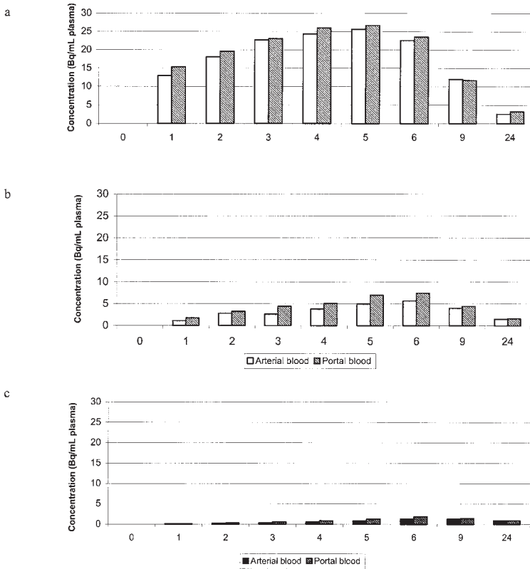
Figure 3. Portal and arterial kinetics of 14 C phenanthrene (a), 14 C benzo[a]pyrene (b) and 14 C 2,3,7,8-TCDD (c) in the growing pig after milk ingestion.
