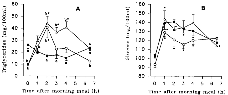
Fig 2. Effect of diet on postprandial plasma concentration of triglycerides (A) and glucose (B) for animals on control (■), soybean (Δ), and lupin (○) diets. a,b P \leq 0.05 between diets, * P \leq 0.05 compared to preprandial values. Vertical bars are standard errors.
