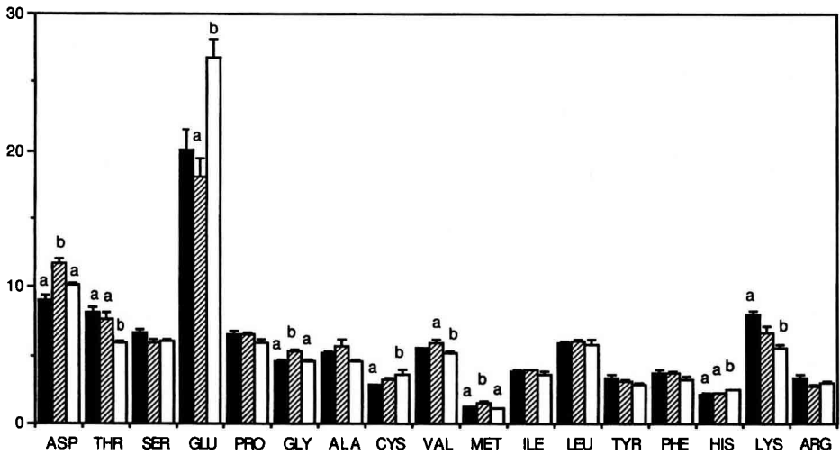
Fig 4. Amino-acid composition (% of assayed AA) of ileal digesta with the control (■), soyabean (▨) or lupin (□) diets. a,b P \leq 0.05 between means with different letters. Vertical bars are standard errors.
