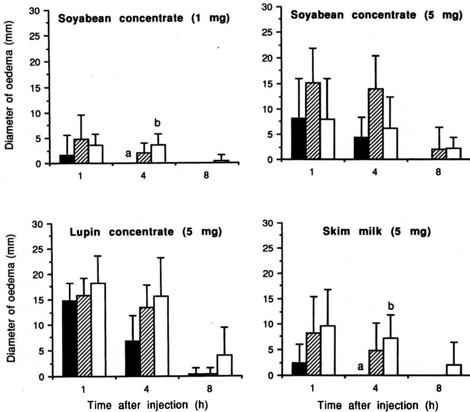
Fig 3. Skin responses of calves following the injection of the 2 protein concentrates and skim-milk protein for animals on control (■), soyabean (▨), and lupin (□) diets. a,b P \leq 0.05 between means with different letters. Vertical bars are standard errors.
