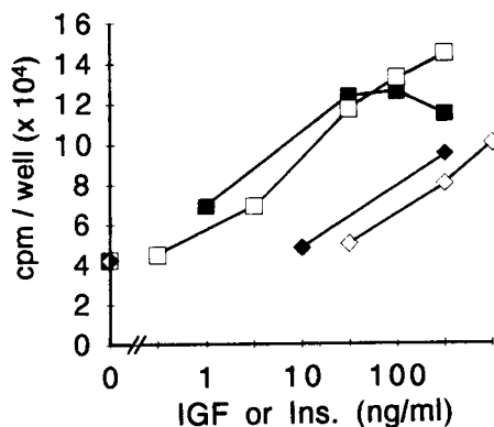
Fig 2. Effect of increasing concentrations of rhIGF I and II, s- and b-insulin on in vitro ^3 H-T incorporation (incubation for 3 d; 8 \mu Ci/ml ^3 H-T and 3rd day) by trout germ cells ( 0.7 \times 10^6 Go + Ci/well). Mean \pm SD ( n = 4 ). —■— IGF-I; —□— IGF-II; —◆— s-insulin; —◇— b-insulin.
