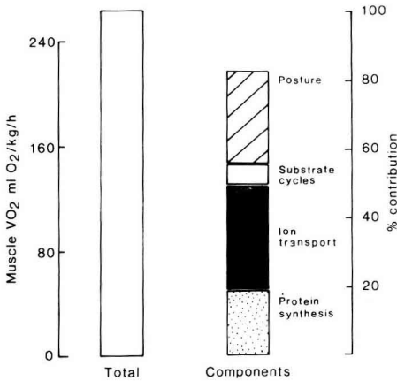
Fig 3. Contribution of specific processes to sheep hindquarter energy expenditure in vivo . Data based on total oxygen uptake across hind-leg muscle of 35-kg lambs at maintenance intake (from Harris et al , 1989).
