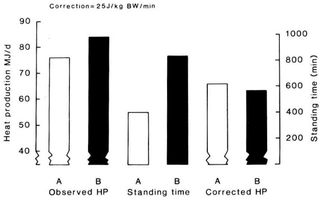
Fig 2. Effect of standing on energy expenditure in cattle. Two Hereford x Friesian heifers (A, 570 kg; B, 590 kg) offered same diet quantity (1.8 x maintenance). Observed heat production corrected for standing time (25 J/kg body wt/min; Brockway, 1987). Data from Mollison and Brockway (unpublished).
