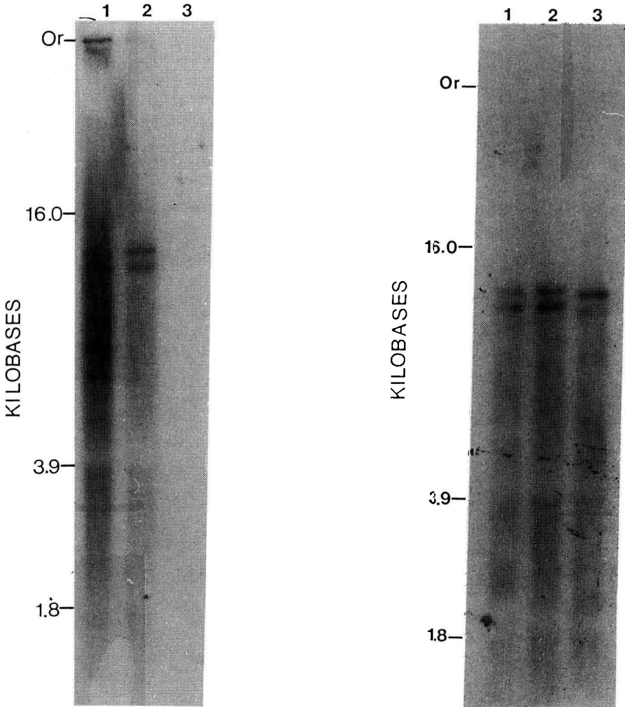
Fig. 8. The long and short FAS mRNAs from goose liver and goose uropygial gland contain the polypyrimidine tract; neither FAS mRNA from duck liver contains this sequence. Poly (A + ) RNA (15 \mu g) was subjected to electrophoresis in a 0.8% agarose gel buffered with morpholinepropane-sulfonic acid (Back et al. , 1986) blot-transferred onto nitrocellulose membrane and hybridized to a synthetic 32 P-labeled polypyrimidine oligonucleotide (40mer) under aqueous conditions (left panel). The blot was washed to remove the probe and rehybridized with 32 P-labeled, single-stranded cDNA generated from M13GFAS3B (right panel). Sources of the RNAs were : lane 1, goose uropygial gland; lane 2, goose liver; lane 3, duckling liver.
