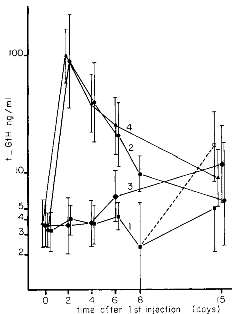
FIG. 2. — Mean plasma gonadotropin level (t-GTH) in the 4 experimental groups.
