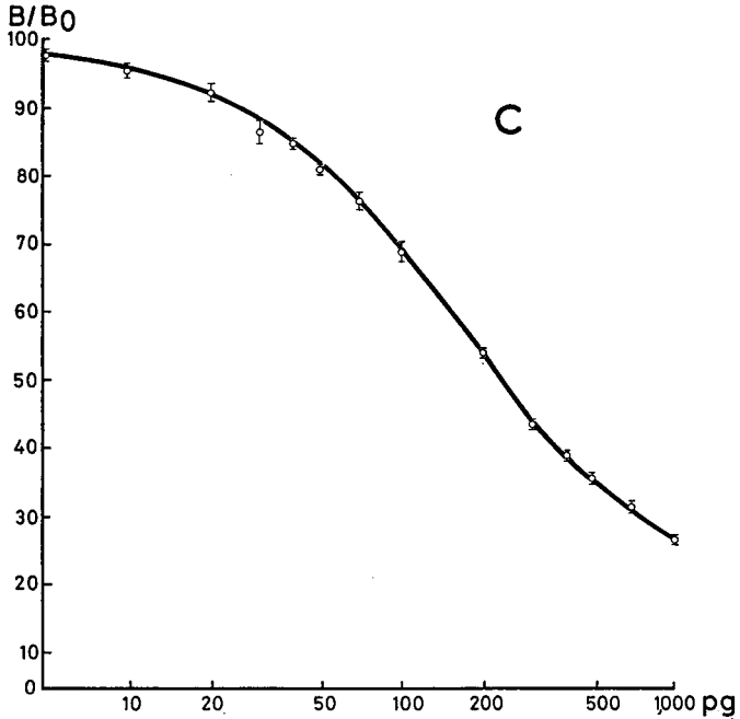
FIG. 3. — Standard curves for the radioimmunoassays of testosterone (A), of 5 \alpha -DHT (B) and of DHA (C). T and DHA standard curves are prepared with 0.05 ml of steroid-free ram plasma ( m \pm \text{sem} ).
