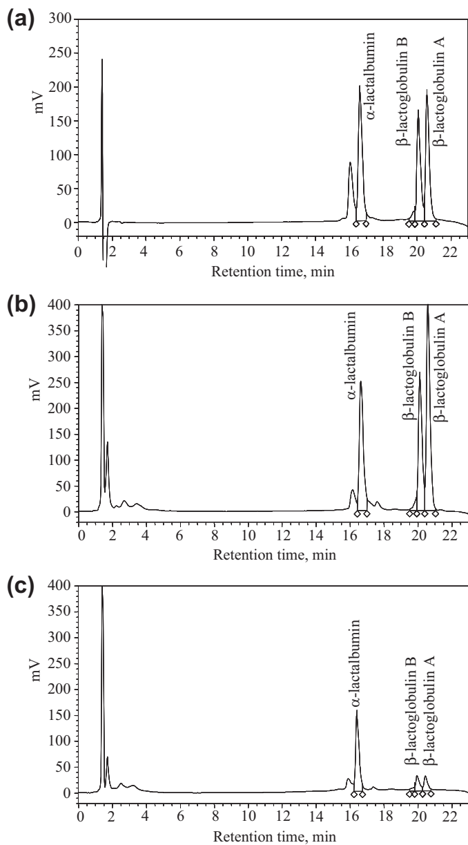
Figure 2. RP-HPLC chromatograms of a standard mixture of \alpha -lactalbumin (0.8 \mu g) and \beta -lactoglobulin (1.6 \mu g) per 10 \mu L injection volume each (a), and of acid-soluble whey proteins in low-heated (b) and high-heated (c) ESL milk samples, having native \beta -Lg contents of 2792 and 260 \text{mg}\cdot\text{L}^{-1} milk, respectively (Nos. 127 and 31).
