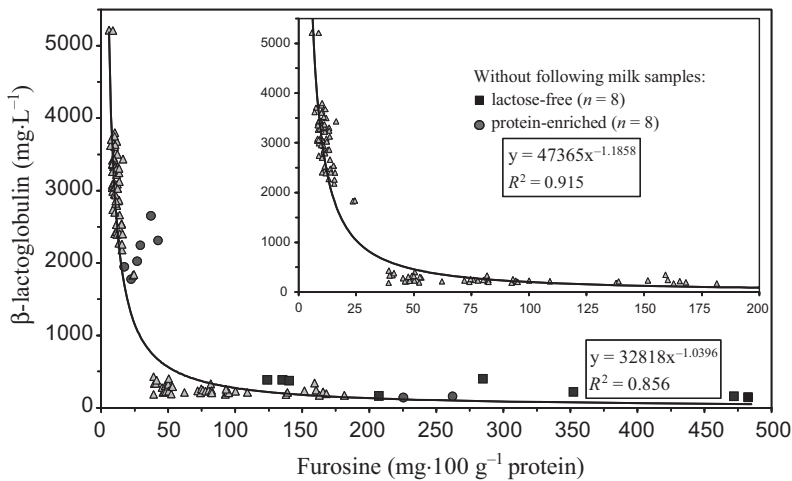
Figure 5. Relationship between acid-soluble \beta -Lg ( \text{mg}\cdot\text{L}^{-1} ) and furosine ( \text{mg}\cdot 100\text{ g}^{-1} protein) contents of milk samples taken from retail outlets in Austria ( n = 128 ).
