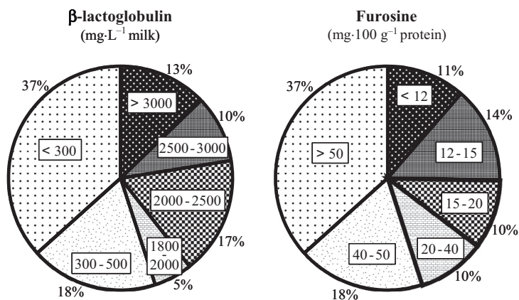
Figure 6. Relative distribution of acid-soluble \beta -Lg (mg·L -1 ) and furosine (mg·100 g -1 protein) contents in ESL milk samples taken from retail outlets in Austria ( n = 71 ).
