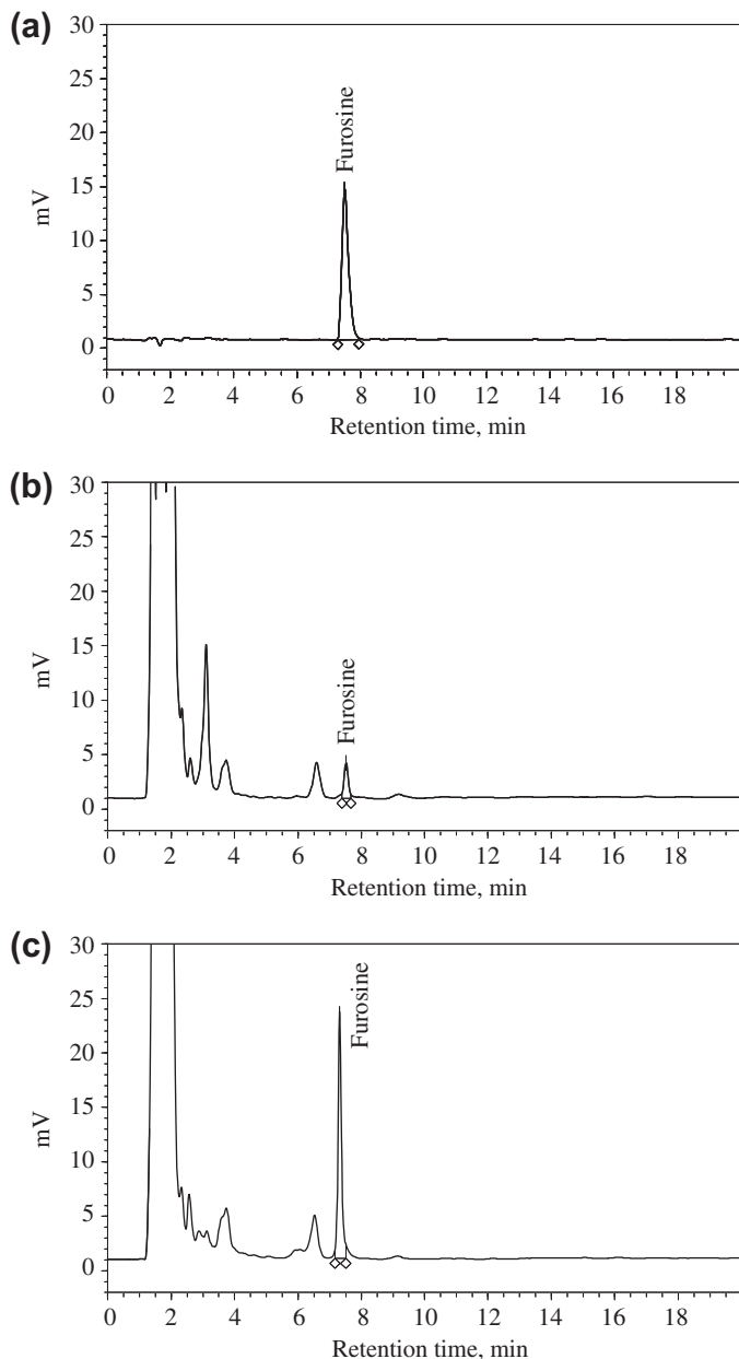
Figure 3. RP-HPLC chromatograms of a furosine standard with 80 pmol per 20 \mu\text{L} injection volume (a), and of furosine in low-heated (b) and high-heated (c) ESL milk samples, having furosine contents of 11.6 and 74.7 \text{mg}\cdot 100\text{ g}^{-1} protein, respectively (Nos. 127 and 31).
