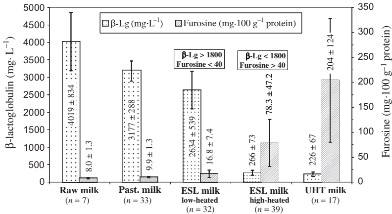
Figure 4. Mean values ( \pm SD) for acid-soluble \beta -Lg ( \text{mg}\cdot\text{L}^{-1} ) and furosine ( \text{mg}\cdot 100\text{ g}^{-1} protein) contents in different categories of heat-treated milk samples taken from retail outlets in Austria ( n = 128 ).
