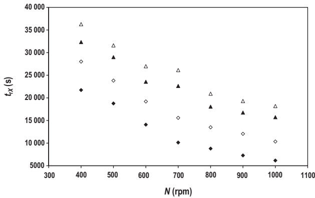
Figure 4. Rehydration time t_{rX} as a function of stirring speed N (rpm). \blacklozenge : X = 0.3 ; \diamond : X = 0.5 ; \blacktriangle : X = 0.7 ; \triangle : X = 0.9 . Fixed \phi and \theta values are equal to 4.8% (w/w) and 30 °C, respectively.
