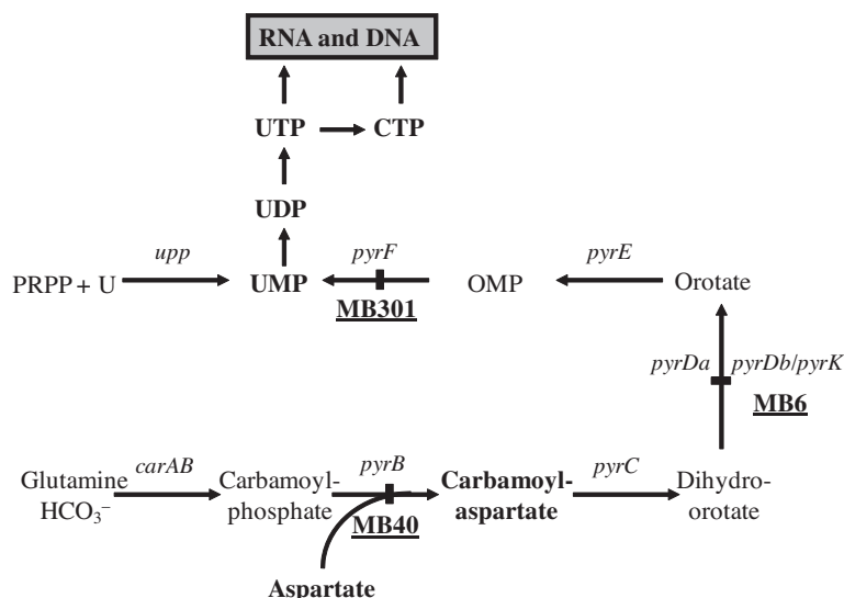
Figure 1. Simplified schematic representation of pyrimidine biosynthesis in L. lactis leading to the central pyrimidine compound UMP that subsequently is converted to UTP and CTP. The genes encoding the enzymes catalyzing the individual reactions are shown. U, uracil; UR, uridine; UMP, uridylylate (monophosphate); OMP, orotidylate (monophosphate); R-1-P, ribose-1-phosphate; PRPP, 5-phosphoribosyl-1- \alpha -pyrophosphate; carAB , carbamoylphosphate synthase; pyrB , aspartate transcarbamoylase; pyrC , dihydroorotase; pyrD , dihydroorotate dehydrogenase; pyrE , orotate phosphoribosyltransferase; pyrF , OMP decarboxylase; upp , uracil phosphoribosyltransferase. MB40, MB6, and MB301 are the three mutant strains lacking the enzymatic activities corresponding to their position.
