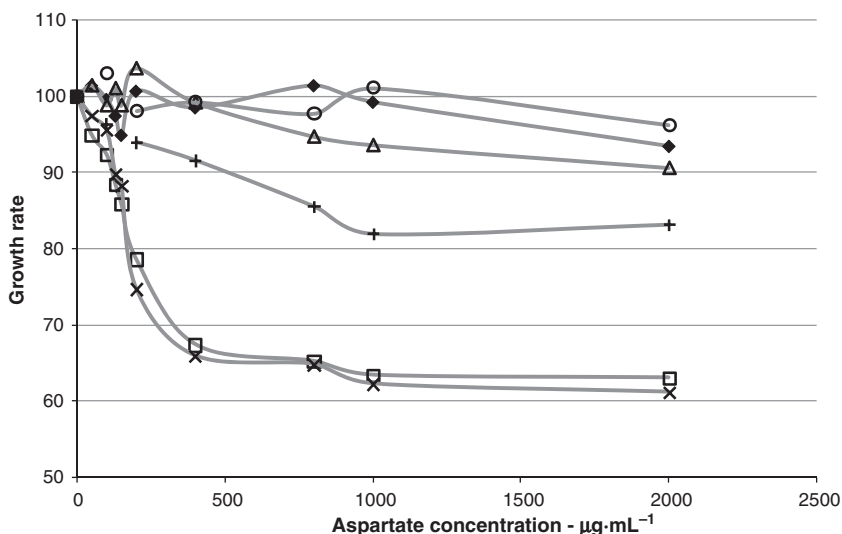
Figure 2. The effect of aspartate on the growth rate of different L. lactis subsp. cremoris strains in GSA. Growth rates are given as the percentage of the growth rate obtainable in GSA without aspartate. The relative growth rates are the mean values of two independent experiments. The standard deviation was 2.6% or better. ◆, MG1363; □, MB6 ( pyrDa and pyrK ); △, MB40 ( pyrB ); ×, MB301 ( pyrF ); +, LM0230; and ○, C2.
