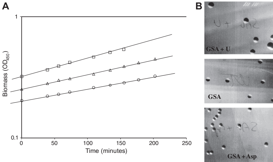
Figure 3. Growth of L. lactis LM0230 on GSA, containing either 0.2 mg·mL -1 of aspartate (GSA + Asp) or 0.02 mg·mL -1 of uracil (GSA + U). (A) A representative example of a growth experiment in liquid medium, supplied with □, uracil; △, nothing; or ○, aspartate. (B) Plates containing same medium. The plates were incubated at 30 °C for 24 h.
