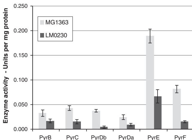
Figure 4. The activities of the enzymes in the pyrimidine biosynthetic pathway. PyrB, aspartate transcarbamoylase; PyrC, dihydroorotase; PyrDa, dihydroorotate dehydrogenase A; PyrDb, dihydroorotate dehydrogenase B complex; PyrE, orotate phosphoribosyltransferase; PyrF, OMP decarboxylase activities were determined in LM0230 (dark gray columns) and MG1363 (light gray columns). The activity of the individual enzymes is given in units per milligram protein in crude extracts. One unit is defined as 10^{-9} mol substrate converted in 1 min.
