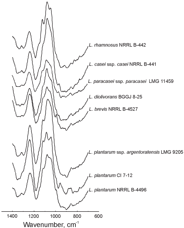
Figure 1. The 1400–700 \text{cm}^{-1} region of FTIR spectra (KBr tablets, 3 mg of biomass) of selected Lactobacillus strains cultivated on MRS agar (30 °C for 48 ± 1 h).
