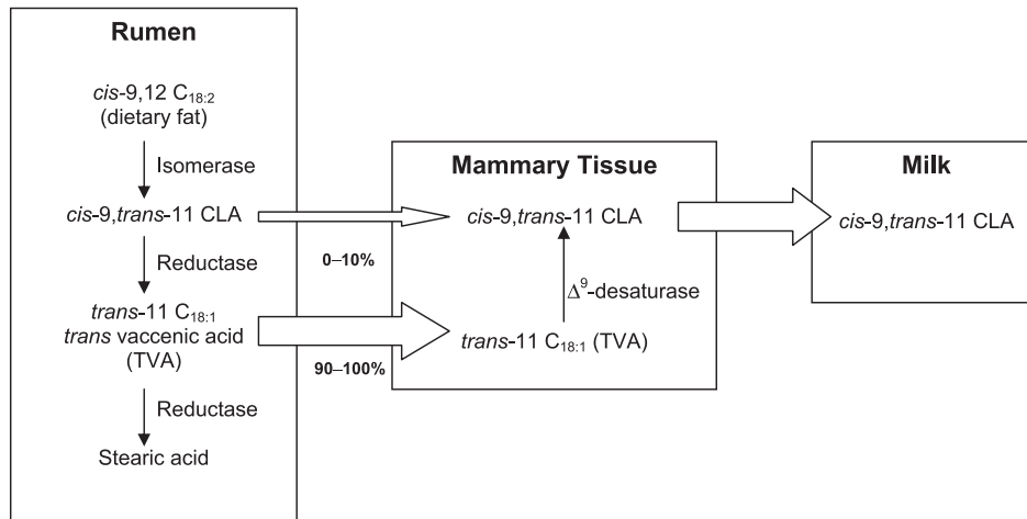
Figure 1. Production of cis-9,trans-11-C 18:2 in ruminant fat by biohydrogenation and tissue \Delta^9 -desaturase (a multienzyme complex that introduces a cis double bond between carbons 9 and 10 of fatty acids [2,18]).
