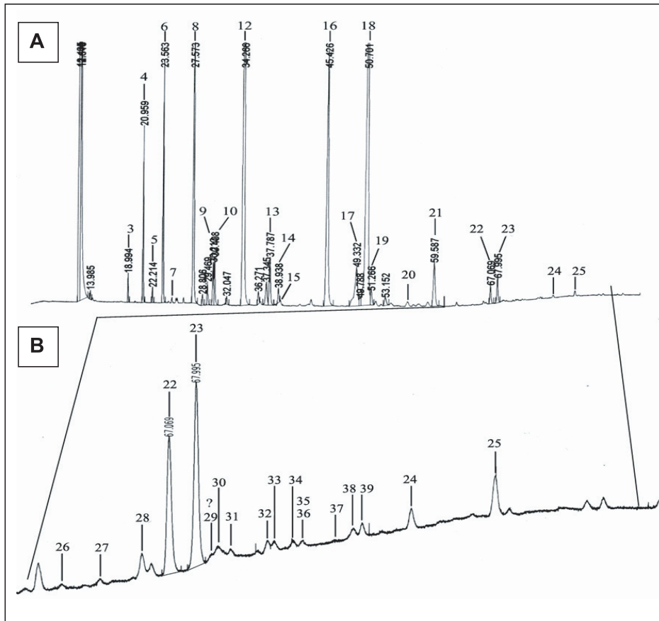
Figure 3. Azorean UHT milk FAME profile. Analytical conditions: Column CP-Sil 88, 100 m \times 0.25 mm i.d., 0.2- \mu m film. Column temperature 60 ^{\circ} C (2 min hold), 175 ^{\circ} C at 20 ^{\circ} C \cdot min ^{-1} (50 min hold), 220 ^{\circ} C at 4 ^{\circ} C \cdot min ^{-1} (30 min hold). Injector 250 ^{\circ} C and detector (FID) 300 ^{\circ} C. Flow 1.66 mL \cdot min ^{-1} (helium), inlet pressure 180 kPa, split ratio 45:1. Legend: (A) Total profile of FAME: 3 – C8:0, 4 – C10:0, 5 – C11:0, 6 – C12:0, 7 – C12:1, 8 – C14:0, 9 – C14:1, 10 – C15:0, 11 – C15:0 (iso), 12 – C16:0, 13 – C16:1, 14 – C17:0, 15 – C17:1, 16 – C18:0, 17 – C18:1 ( trans isomers), 18 – C18:1 (c9), 19 – C18:1 (c7), 20 – ?, 21 – C18:2 (c9,12), 22 – C18:3 (c9,12,15), 23 – C18:2 (c9,t11)-CLA, 24 – C21:0, 25 – ?. (B) Chromatogram expansion between 60 and 80 min: 26 – C20:0, 27 – C20:1 (c11), 28 – C18:3 (c6,9,12), 29 – C18:2 (t8,c10)-CLA, 30 – ?, 31 – C18:2 (t10, c12)-CLA, 32 – C18:2 (c8,10)-CLA, 33 – C18:2 (c9,11)-CLA, 34 – C18:2 (c10,12)-CLA, 35 – C18:2 (c11,13)-CLA, 36 – C20:2 (c11,14), 37 – C18:2 (t11,13)-CLA, 38 – C18:2 (t8,10 + t9,11 + t10,12)-CLA, 39 – C20:3 (c8,11,14).
