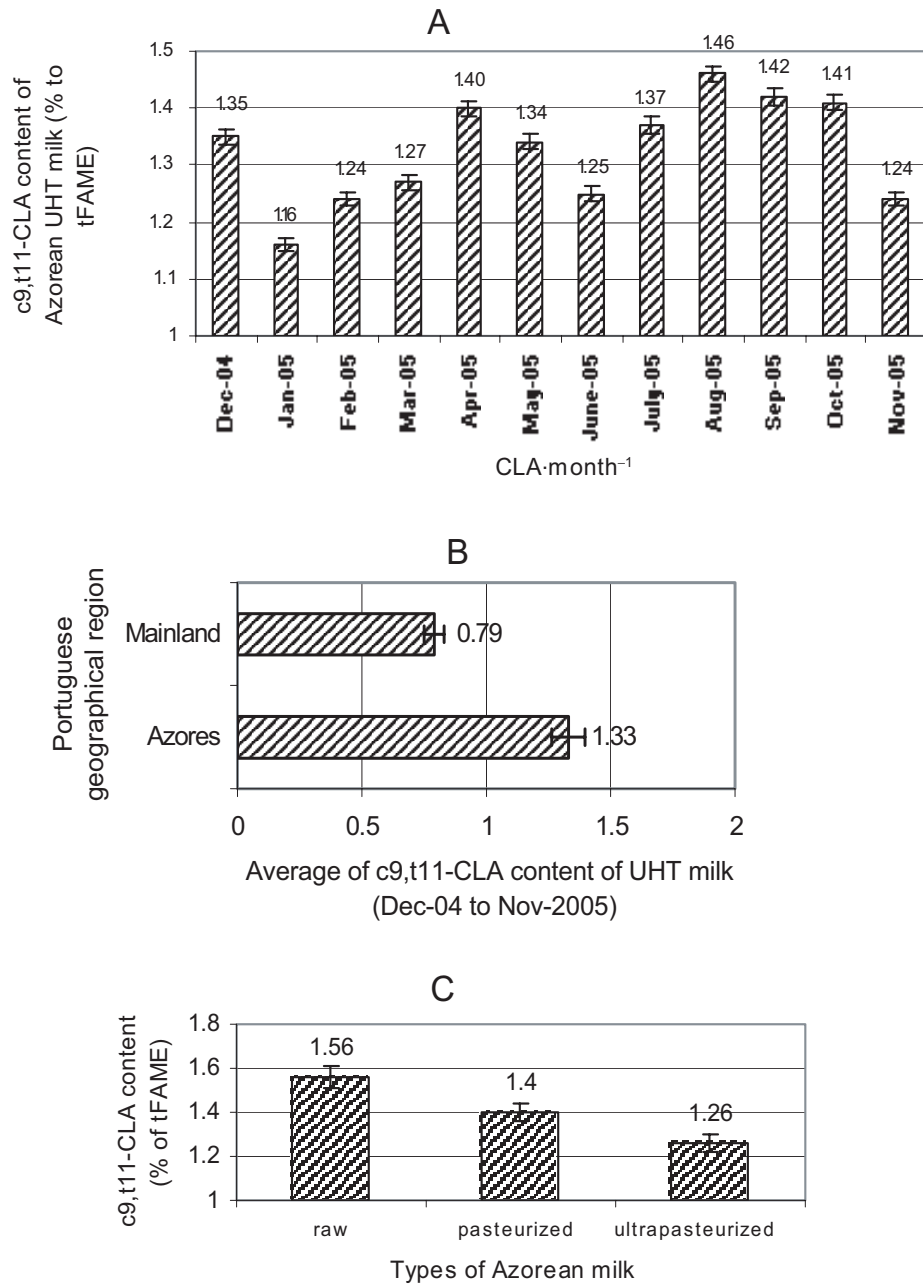
Figure 4. A. Variability in the cis -9, trans -11-CLA isomer content of Azorean UHT milk throughout the year (2005). B. Comparison of the cis -9, trans -11-CLA isomer content of Azorean UHT milk versus Portuguese mainland UHT milk. C. Effect of processing temperatures (pasteurization and ultrapasteurization) on the cis -9, trans -11-CLA content of Azorean UHT milk.
