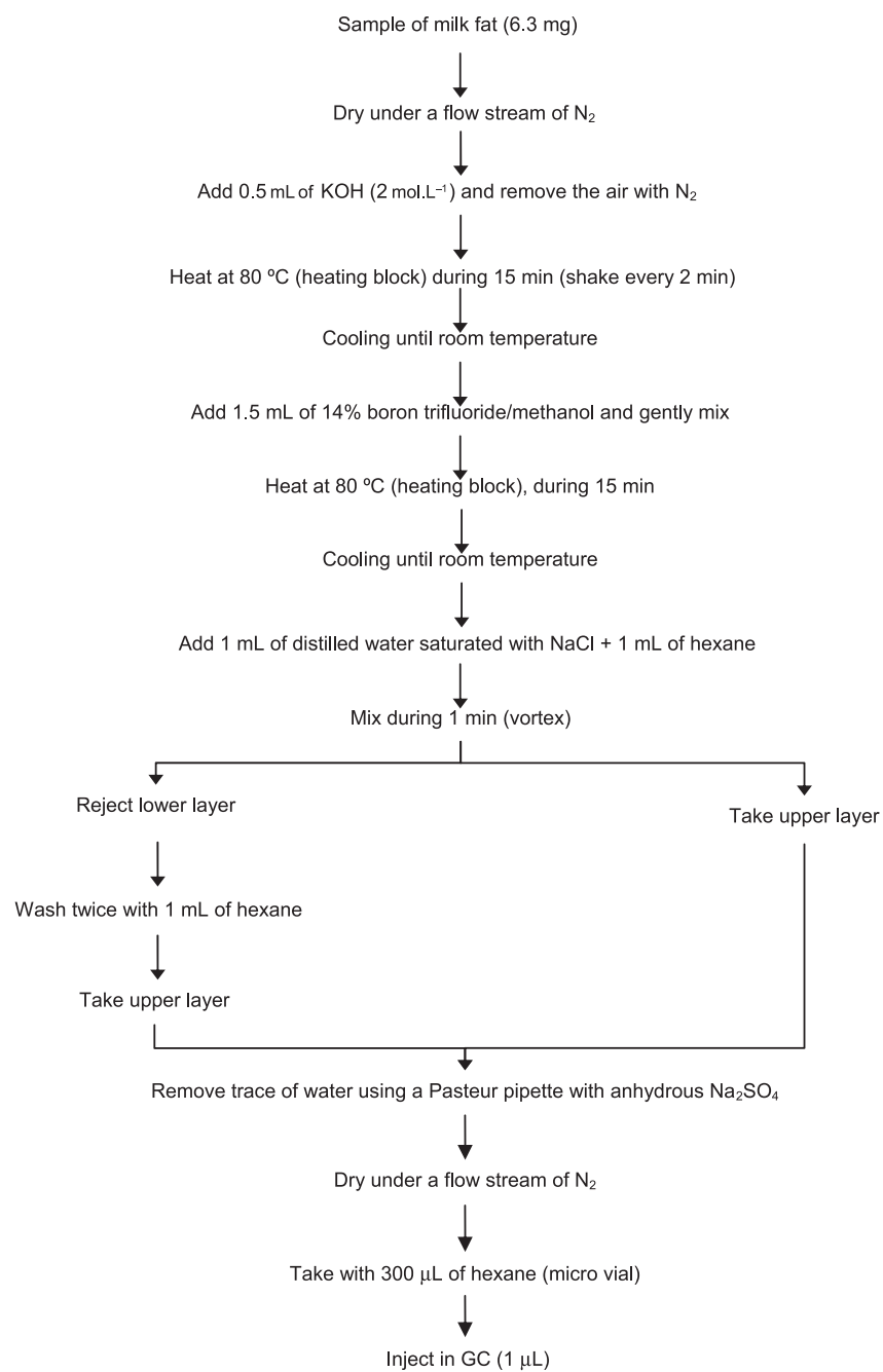
Figure 2. Protocol of the milk fat methylation procedure.
