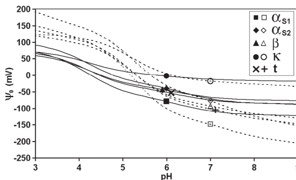
Figure 15. Evolution of the electrostatic surface potential ( \psi_0 ) of principal casein fractions ( \alpha_{S1^-} , \alpha_{S2^-} , \beta - and \kappa -) dissolved in water (solid lines) or in 60% (v/v) ethanol (broken lines) as a function of pH. The lines (t) represent total casein.
