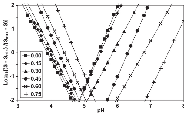
Figure 2. The effect of pH (3–8) and ethanol volume fraction (0–0.75) on the solubility profile of 10 g·L -1 sodium caseinate solutions. Solid lines represent Equation (3) with coefficients pH 1 and D presented in Figure 3 and Table II.
