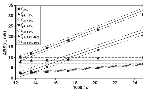
Figure 14. Absolute value of the zeta potential ( \zeta ) of casein monomers as a function of the reciprocal relative dielectric constant ( 1/\epsilon ) for the line \text{pH}_0 ( \zeta_{0\%} ), from Figure 3 and the isolines \text{pH}_{1:10\%} , \text{pH}_{2:10\%} , \text{pH}_{1:90\%} and \text{pH}_{2:90\%} from Figure 4, corresponding to casein solubilities of 10% and 90% for the pH range below ( 1 ) and over ( 2 ) the minimal zeta potential ( \zeta ). Solid lines represent Equation (5) with coefficients A and B given in Table V and broken lines show standard deviation limits.
