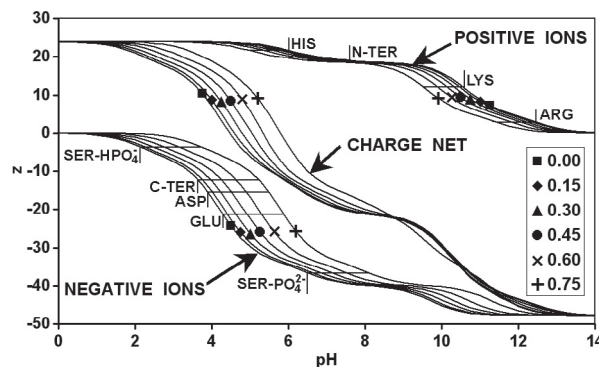
Figure 5. Evolution of the electrical charge ( z ) of total casein monomers, as a function of pH and ethanol volume fraction (0 to 0.75), calculated by Equations (3) and (4) with \gamma = 1 and pK taken from Walstra and Jenness [75]. Horizontal lines with amino acid name abbreviations representing their apparent pK evolution as a function of the ethanol volume fraction (0–0.75).
