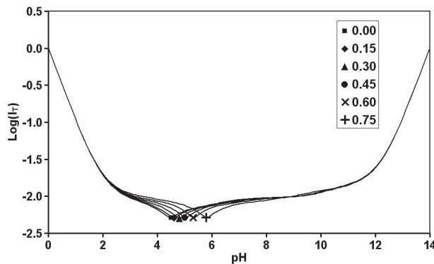
Figure 7. Evolution of the logarithm of the total ionic strength ( I_T in \text{mol}\cdot\text{L}^{-1} ), as a function of pH and ethanol volume fraction (0 to 0.75), calculated using Equation (1).
