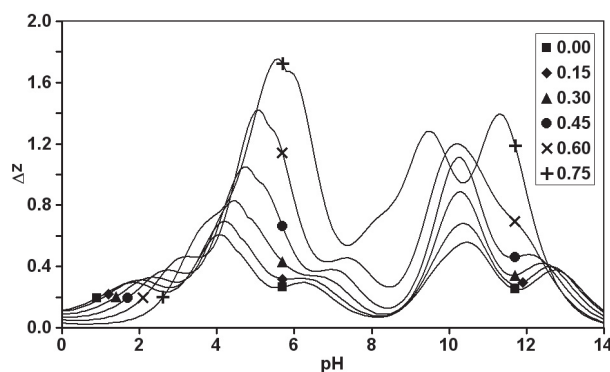
Figure 9. Evolution of the difference ( \Delta z = z_{\gamma=1} - z_{\gamma} ) between the net electrical charge ( z ) of total casein monomers, calculated by Equations (3) and (4) for the activity coefficient \gamma = 1 and for the values of \gamma taken from Figure 8, as a function of pH and ethanol volume fraction (0 to 0.75).
