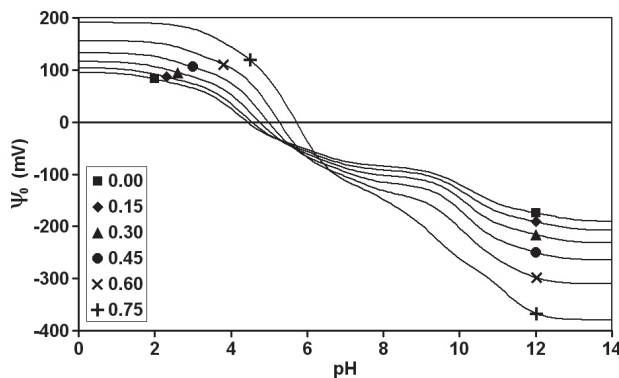
Figure 10. Evolution of the electrostatic surface potential ( \psi_0 ) of sodium caseinate monomers, as a function of pH and ethanol volume fraction (E), calculated by Equation (9) with the charge (z) calculated by Equations (3) and (4) and the activity coefficient ( \gamma ) by Equation (2).
