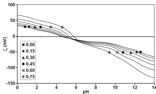
Figure 13. Evolution of the zeta potential ( \zeta ) of casein monomers, as a function of pH and ethanol volume fraction (0 to 0.75), calculated by Equation (10) for T = 293 K.
