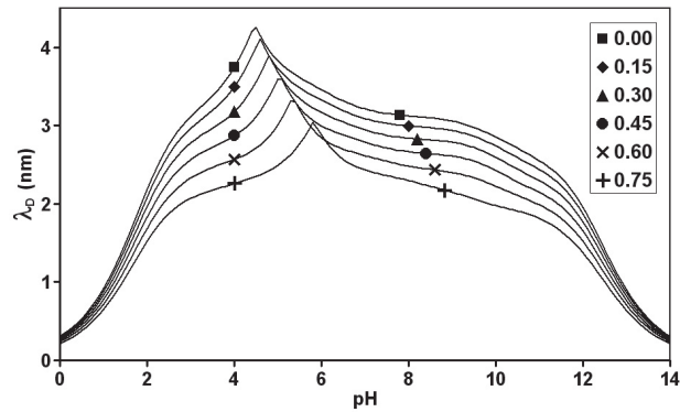
Figure 12. Evolution of the Debye length ( \lambda_D ), as a function of pH and of ethanol volume fraction (0 to 0.75), calculated by Equation (11) for T = 293 K.
