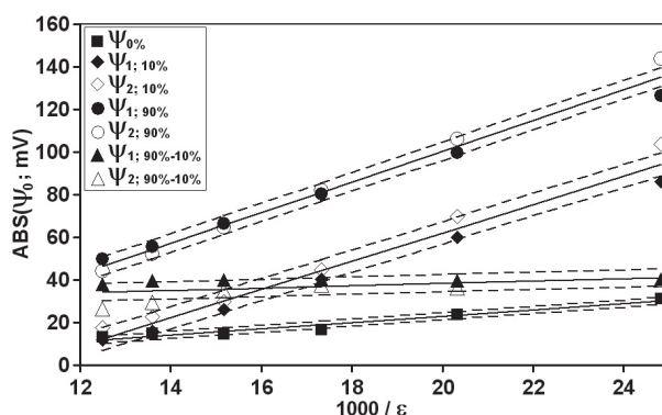
Figure 11. Absolute value of the electrostatic surface potential ( \psi_0 ) of casein monomers as a function of the reciprocal relative dielectric constant ( 1/\epsilon ) for the line pH_0 , from Figure 3 ( \psi_0\% ) and for the isolines pH_{1;10\%} , pH_{2;10\%} , pH_{1;90\%} and pH_{2;90\%} from Figure 4, corresponding to casein solubilities of 10% and 90% for the pH range below (1) and over (2) the minimal surface potential ( \psi_0 ). Solid lines represent Equation (5) with coefficients A and B given in Table IV and broken lines show standard deviation limits.
