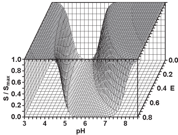
Figure 4. Relative casein solubility ( S/S_{\text{max}} ) as a function of pH and ethanol volume fraction (E), calculated by Equation (8) with S_{\text{min}} = 0 , S_{\text{max}} = 100 and with average \text{pH}_{50\%} and D coefficients calculated by the regression equations from Table II.
