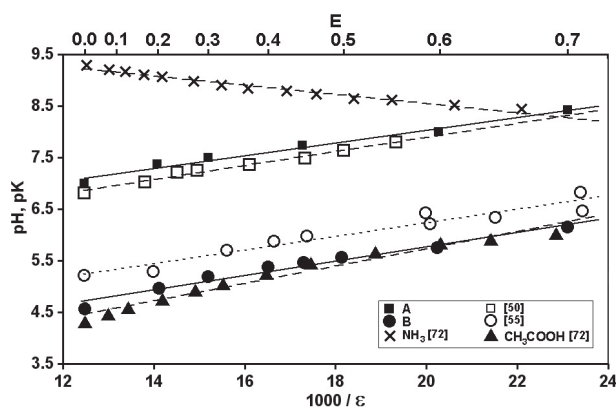
Figure 1. The pH shift of sodium caseinate in water / ethanol solutions as a function of the reciprocal relative dielectric constant ( \epsilon ): E = ethanol volume fraction. (■) – 10 g·L -1 sample (A) – initial pH 7.0; (□) – 30 g·L -1 sodium caseinate [50]; (●) – 10 g·L -1 sample (B) = sample A with initial pH adjusted to 4.6; (○) – minimum ethanol stability of sodium caseinate [55]; (▲) – apparent pK of acetic acid [72]; (×) – apparent pK of ammonium [72]. Solid, broken and dotted lines represent equation (1) with coefficients A and 1/B given in Table I.
