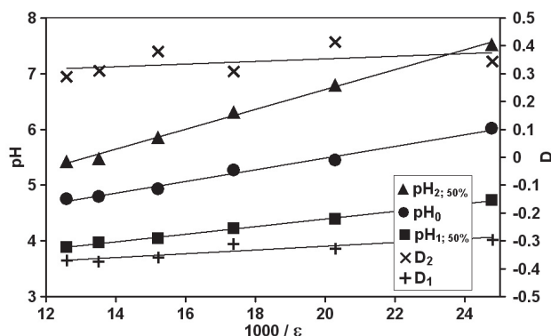
Figure 3. Evolution of pH corresponding to 50% casein solubility (pH 1,50% and pH 2,50% ) and coefficient D from Equation (3) as a function of the reciprocal relative dielectric constant (1/ε) for the pH range below (pH 1 and D 1 ) and over (pH 2 and D 2 ) the minimal solubility point (pH 0 ). Solid lines represent Equation (1) with coefficients A and B given in Table II.
