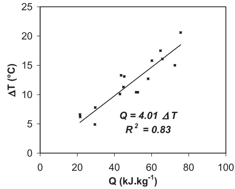
Figure 2. Relationship between the amount of energy ( Q in \text{kJ}\cdot\text{kg}^{-1} ) and the temperature increase ( \Delta T in °C) during one passage of the product through the treatment cell.
