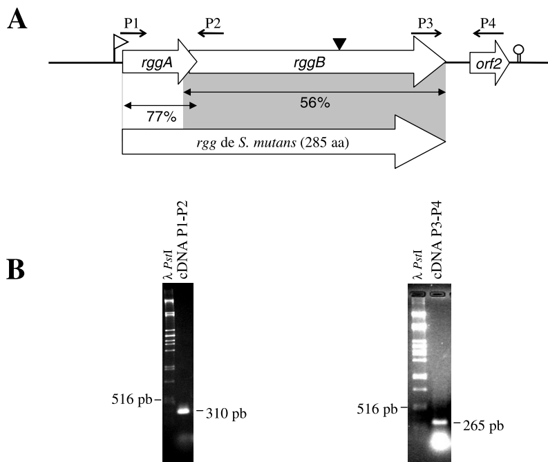
Figure 2. Organisation of the rgg locus of S. thermophilus CNRZ368. (A) The solid line symbolises the S. thermophilus genomic DNA. ORFs are indicated as open arrows. The black arrowhead indicates the insertion site of pGh9:ISS1 within the genome of the 15H7 mutant. The open flag indicates the putative promoter and the putative rho-independent terminator is represented as a hairpin loop. Grey boxes symbolise the homologous region between rgg from S. thermophilus and from S. mutans : the percentage of amino acid identity is indicated below the double arrows. Primers used for RT-PCR experiments are indicated. The expected size of the P1-P2 and P3-P4 PCR fragments is 310 pb and 265 pb, respectively. (B) Gel electrophoresis showing the RT-PCR products obtained using the primers P1-P2 and P3-P4.
