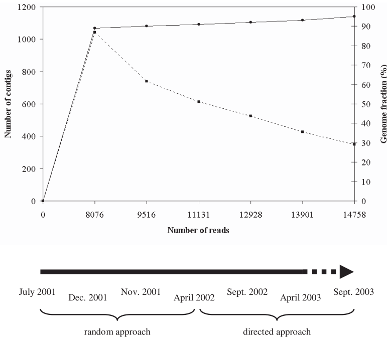
Figure 1. Progress of the sequencing project. The full line corresponds to the increasing genome fraction, while the dashed one is the decreasing number of contigs. The arrow corresponds to the progress of the sequencing project in time.
