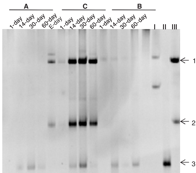
Figure 2. Identification of bacterial species present throughout the cheese-making processing in the three factories (A, B and C). TGGE was performed with the 16S-23S-spacer region rDNA fragment that was PCR amplified from extracts of enriched raw ripened milk (E-Day) and cheeses at different times of ripening (1-day, 14-day, 30-day and 60-day). Lane I: Lactobacillus delbrueckii subsp. bulgaricus CNRZ 225; lane II: Lactobacillus paracasei subsp. paracasei CNRZ 763; lane III: Lactobacillus plantarum CNRZ 211. The positions of the bands for the reference strains Lactobacillus plantarum CNRZ 211 (1 and 2) and Lactobacillus paracasei subsp. paracasei CNRZ 763 (3) are indicated by arrows.
