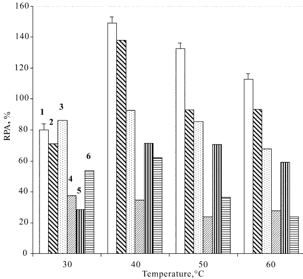
Figure 3. Relative proteolytic activity (RPA, %) of the \beta -gal-containing CCEs from three thermophilic dairy cultures during lactose hydrolysis in 10 or 30% (w/w) skim milk preparation performed at different temperatures (numbers on top of bars indicate CCE containing reaction systems as follows: 1 = Lb11842: Lb. delbrueckii ssp. bulgaricus 11842 – 10%; 2 = Lb11842: 30%; 3 = St143: St. thermophilus 143 – 10%; 4 = St143 – 30%; 5 = Lb3078: Lb. delbrueckii ssp. lactis 3078 – 10%; 6 = Lb3078 – 30%; same order used for all temperature sets; bars present adjusted standard error of the means; n = 4 or more).
