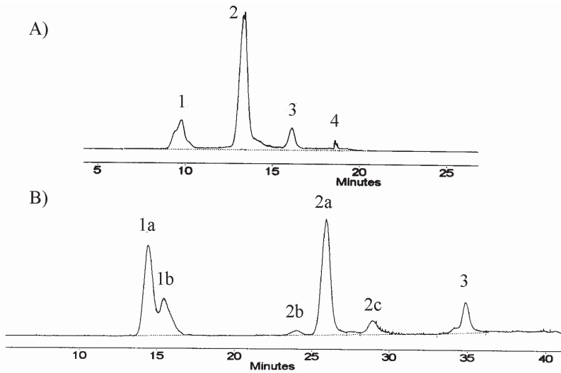
Figure 1. Typical HPLC chromatograms obtained when analyzing products of the lactose hydrolysis by the Lb11842 CCE preparation as acquired by (A) Jordi oligosaccharide or (B) Supelcosil carbohydrate columns (peaks identified as follows: 1 = monosaccharides; 2 = disaccharides; 3 = trisaccharides; 4 = tetrasaccharides; 1a = glucose; 1b = galactose; 2a = lactose; 2b and 2c = unidentified disaccharides).
