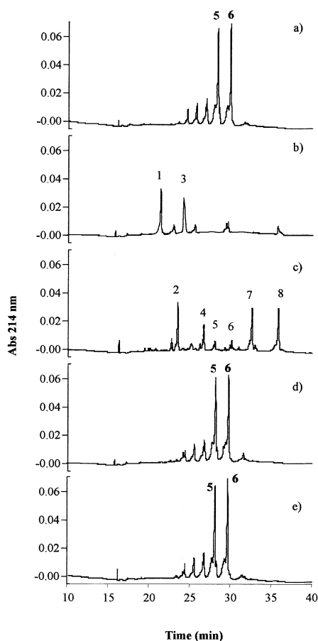
Figure 2. Electropherogram for ovine \beta -casein (a) untreated and incubated during 30 min with (b) plasmin; (c) Cynara cardunculus L.; (d) animal rennet; and (e) microbial coagulant. Peak identification: 1: \gamma_2 -casein; 2: possible peak B; 3: \gamma_3 -casein; 5: \beta_1 -casein; 6: \beta_2 -casein; and 4, 7 and 8: degradation products from the action of the vegetable coagulant on \beta -casein.
