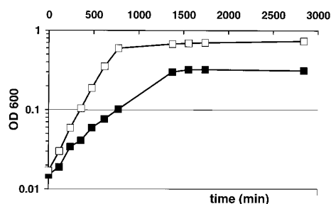
Figure 2. Growth of L. sakei 23K (wild type, bold symbols) and RV2006 ( \Delta ptsI , open symbols) on MCD containing 0.5% ribose.
