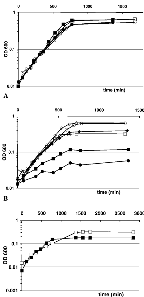
Figure 3. Growth of L. sakei 23K (wild type, open symbols) and RV52 (mannose mutant, bold symbols) on (A) fructose (circles) or sucrose (squares); (B) mannose (circles), glucose 0.1% (squares) or glucose 0.5% (diamonds); (C) ribose. Bacteria were grown in MCD medium containing 0.5% sugars (except glucose 0.1%).
