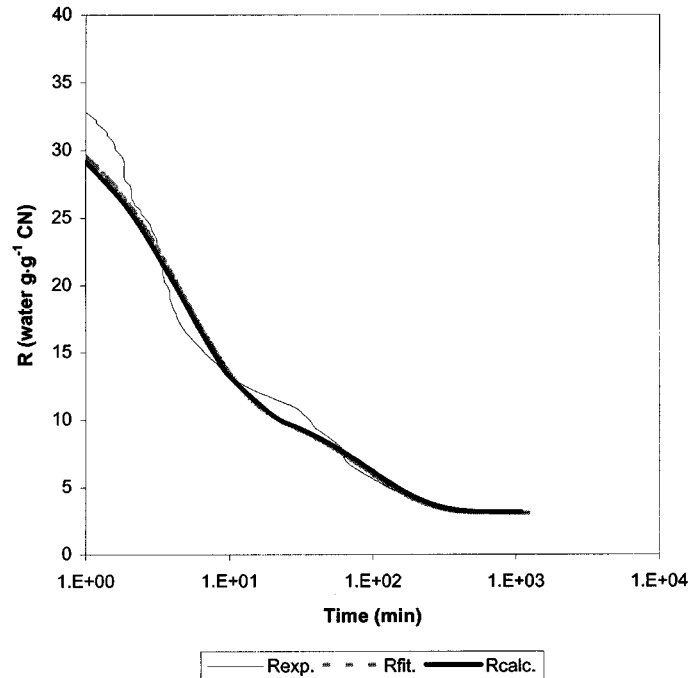
Figure 3. Comparison of R values obtained from experimental data (Rexp.) of a whey drainage kinetics (ren.pH = 6.4, milk CN = 27, IS = 1.0) with: (Rfit.) the fitting to the equation (1), R = R1 \exp(-t/\tau1) + R2 \exp(-t/\tau2) + R3 obtained by the least square method, and with (Rcalc.) the curve calculated from equation (2) keeping into account the average effects of factors CN, IS and ren.pH.
