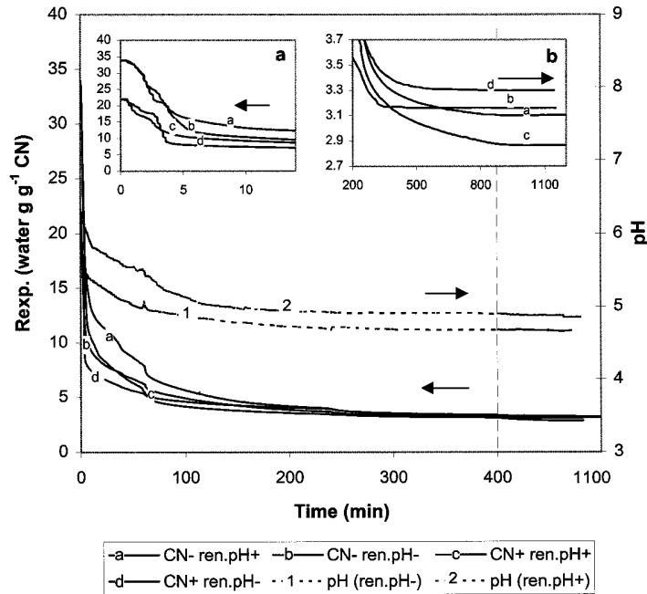
Figure 1. Water content of the draining curd, Rexp. ( \text{g}\cdot\text{g}^{-1} casein), during the course of whey drainage experiments on 4 different milk samples: ren.pH = 6.0 or 6.4 (ren.pH-/+), CN = 27 or 37 \text{g}\cdot\text{kg}^{-1} (CN-/+), IS = 1.0. Expanded scales in the inset. The arrows indicate the reference axes.
