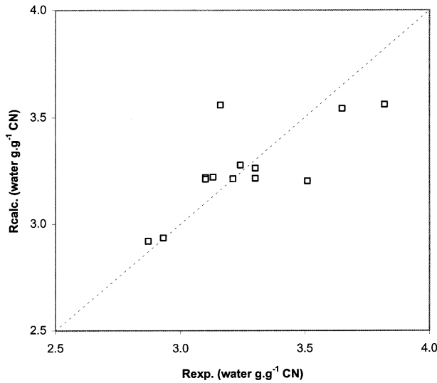
Figure 6. Comparison of the amounts of water in drained curd (Rcalc.), calculated according to equation (2), and (Rexp.), obtained from drainage data. t = 1000 \text{ min} .
