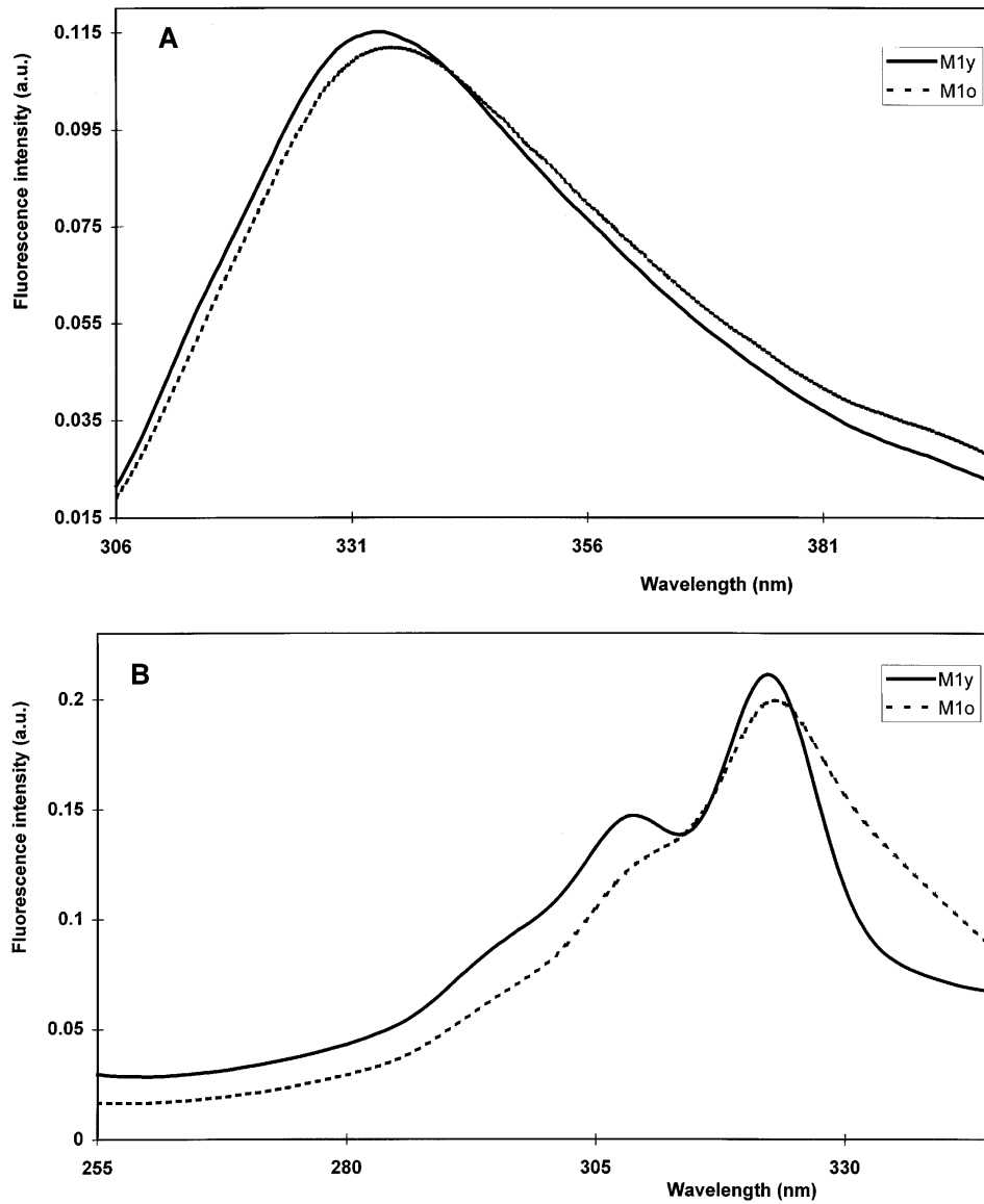
Figure 1. Fluorescence spectra of cheeses: (A) Tryptophan emission and (B) Vitamin A excitation. (—) Mesophilic-I young, (-----) mesophilic-I old cheeses.
