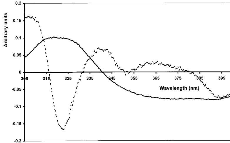
Figure 5. Spectral patterns corresponding to the principal components 1 (—) and 2 (----) of tryptophan data recorded on cheeses (Fig. 4).
