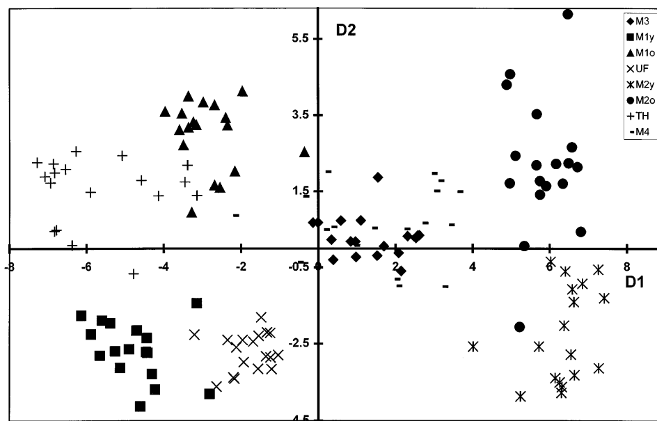
Figure 2. Discriminant analysis similarity map determined by discriminant functions 1 and 2 for the tryptophan spectra of the eight cheeses.
