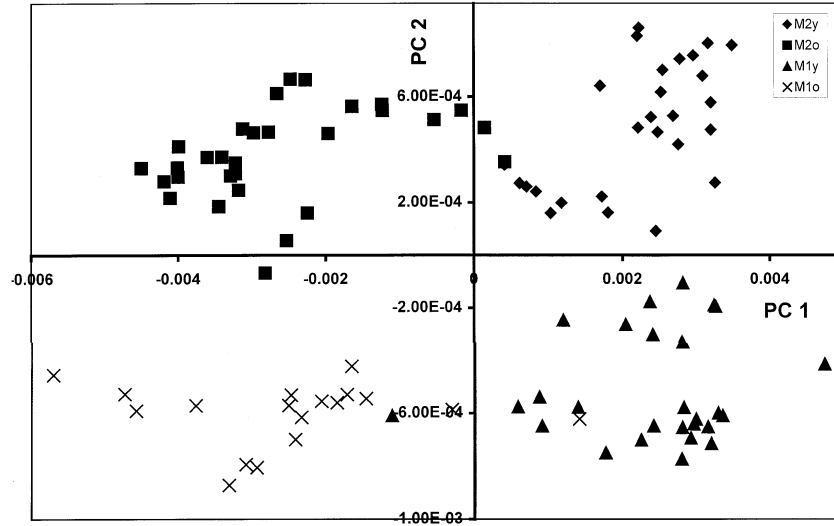
Figure 4. Principal component analysis similarity map determined by principal components 1 and 2 for the tryptophan spectra of mesophilic-I young, mesophilic-I old, mesophilic-II young and mesophilic-II old cheeses.
