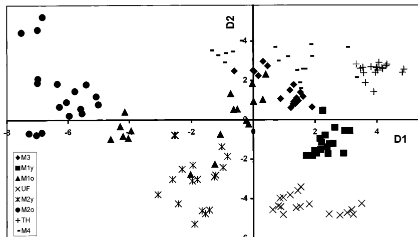
Figure 3. Discriminant analysis similarity map determined by discriminant functions 1 and 2 for the vitamin-A spectra of the eight cheeses.
