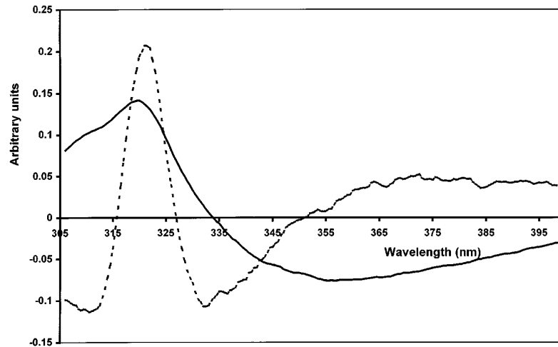
Figure 6. Spectral patterns 1 and 2 corresponding to the principal component 1 (—) and 2 (----) of the principal component analysis performed on the spectral data recorded during rennet, acid-rennet and acid coagulations of milk*.
