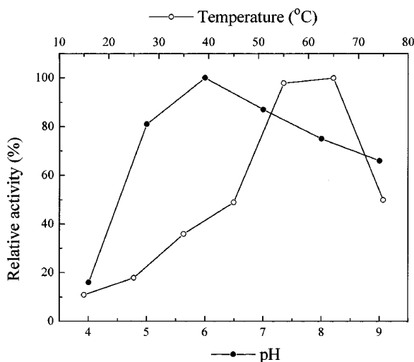
Figure 4. Effect of the pH (●) and the temperature (○) on the esterase from P. freudenreichii ssp. freudenreichii ITG 14, with \alpha -naphthyl-acetate as substrate.
