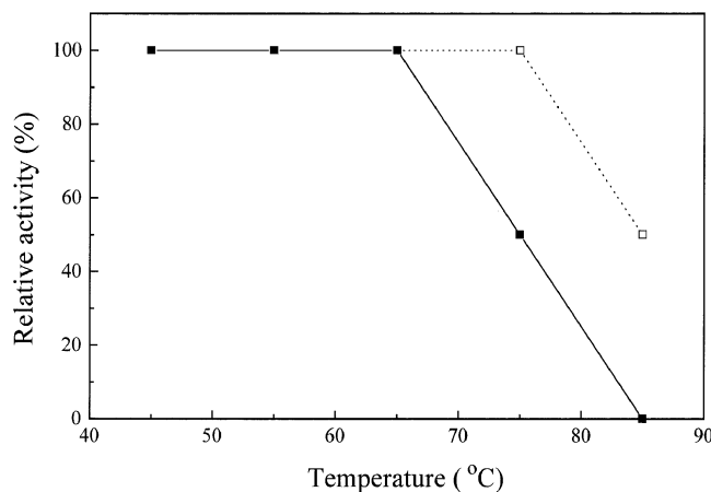
Figure 5. Thermal inactivation of the esterase of P. freudenreichii ssp. freudenreichii ITG 14, in the absence (□) and in the presence (■) of \alpha -naphthyl-acetate as substrate.
