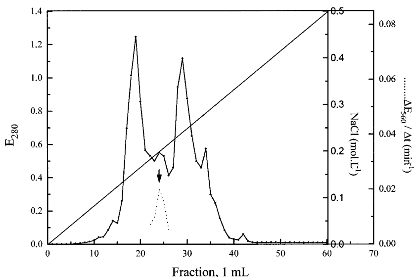
Figure 2. Elution profile of the esterase from the Mono Q HR 5/5 column with a linear gradient of 0\text{--}0.5 \text{ mol}\cdot\text{L}^{-1} NaCl in 50 \text{ mmol}\cdot\text{L}^{-1} Tris:HCl buffer, pH 7.0. Flow rate 1 \text{ mL}\cdot\text{min}^{-1} . Fraction volume 1 \text{ mL} .
