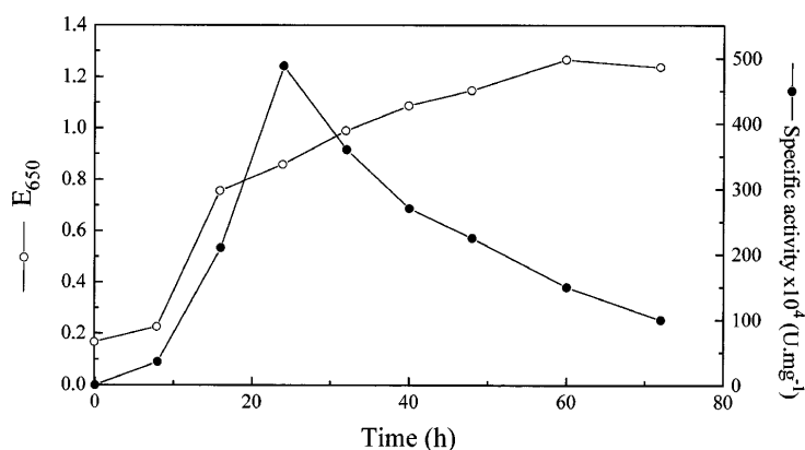
Figure 1. Esterase production during growth of P. freudenreichii ssp. freudenreichii ITG 14.
