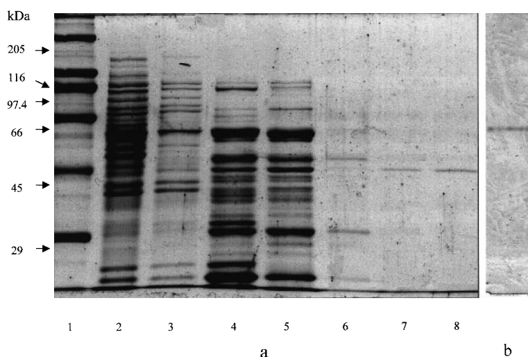
Figure 3. (a) SDS-Polyacrylamide gel electrophoresis (10% acrylamide; 0.025 mol·L -1 Tris-0.19 mol·L -1 glycine buffer, pH 8.3). Lanes: 1, marker proteins; 2, crude cell free extract; 3, after DEAE-cellulose; 4, after Mono Q at pH 8.5; 5, after Mono Q at pH 7.0; 6, 7 and 8, Sephacryl S-300 active fractions 37, 38 and 39, respectively. (b) Polyacrylamide gel electrophoresis without SDS and \beta -mercaptoethanol (10% acrylamide; 0.025 mol·L -1 Tris-0.19 mol·L -1 glycine buffer, pH 8.3): purified esterase reacted with \alpha -naphthyl-acetate and Fast Red TR.
