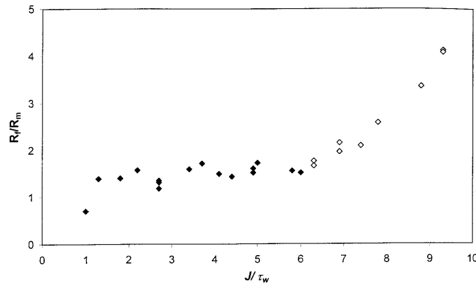
Figure 1. Normalized overall fouling hydraulic resistance ( R_f/R_m ) as a function of the J/\tau_w ratio, for the nanofiltration processes of concentrated sweet whey. VRR 2; 18 °C; FV 20 L·m -2 .
