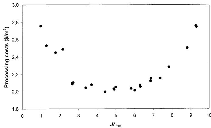
Figure 3. Nanofiltration estimated processing costs ( \$/\text{m}^3 ) as a function of the J/\tau_w ratio. VRR 2; 18 °C; FV 20 \text{ L}\cdot\text{m}^{-2} .
