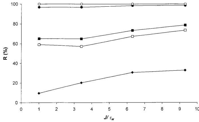
Figure 2. Percentage of rejection R (%) of mineral species during the nanofiltration process of concentrated whey (VRR 2), at 18 °C and for different ratios J/\tau_w ( \text{Ca}^{2+} : ●; \text{Mg}^{2+} : ○; \text{Na}^+ : □; \text{K}^+ : ■; \text{Cl}^- : ◆).
