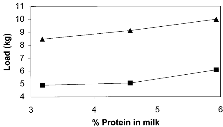
Figure 3. Hardness (▲) and fracturability (■) of cheese as a function of protein concentration in cheese milk. Means averaged across P and all ages.
