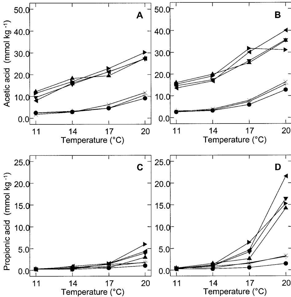
Figure 4. Concentration of acetic acid after 60 days ( A ) after 90 days ( B ), propionic acid after 60 days ( C ) and after 90 days ( D ) at different ripening temperatures in Raclette cheeses made from raw, pasteurised and microfiltered milk and its mixtures. \blacktriangleright raw milk (Ra), \blacktriangleleft + pasteurised milk (Pa), \bullet microfiltered milk (MF), \blacktriangleleft Ra/Pa (50:50%), \blacktriangle Ra/MF (50:50%), \blacktriangledown Ra/Pa/MF (33:33:33%), \times Pa/MF (50:50%). Means of two replicates.
