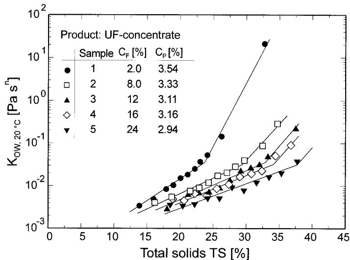
Figure 1. Viscosity coefficient of milk concentrate dependent on the total solids (table inside: fat and protein content prior to concentration [12]).
