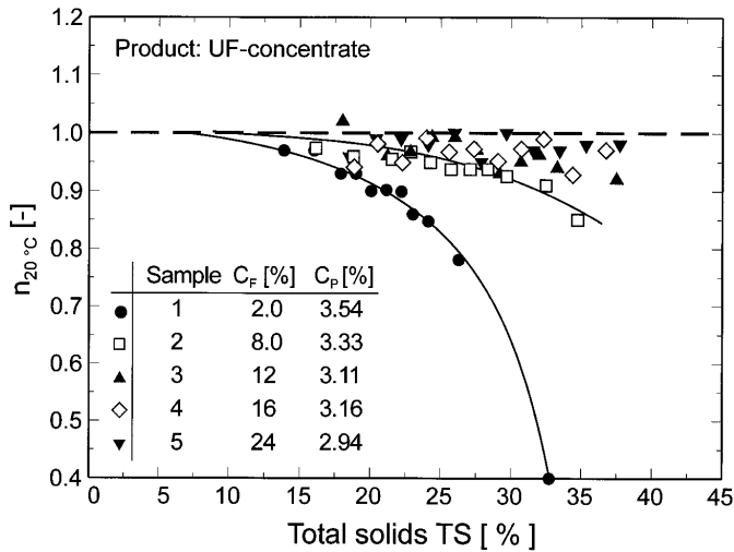
Figure 2. Fluid index of milk concentrates dependent on the total solids for milk [12].
