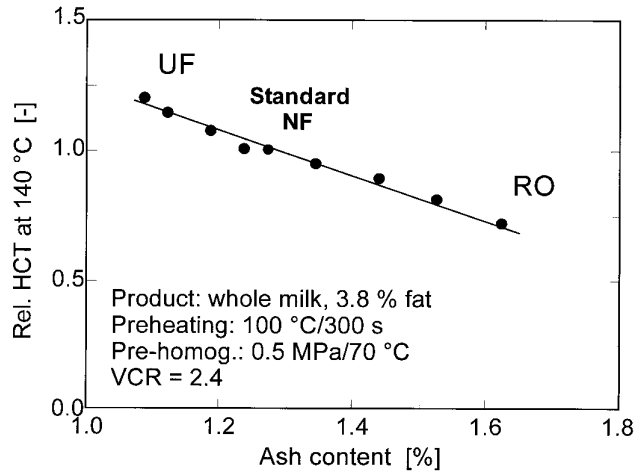
Figure 7. Relative heat coagulation time at 140 °C for mixed milk concentrates (UF: ultrafiltration, NF: nanofiltration, RO: reverse osmosis).
