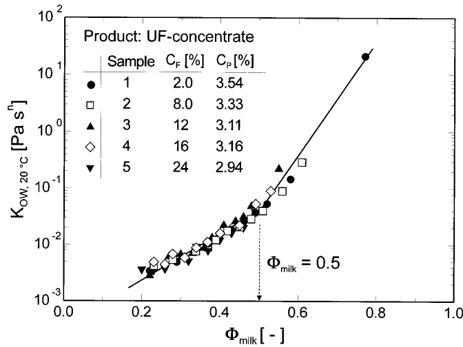
Figure 3. Viscosity coefficient of milk concentrates dependent on the volume fraction for milk [12].
