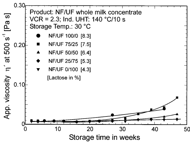
Figure 9. Viscosity increase during storage dependent of the lactose content of the milk concentrates (table inside: e.g. NF/UF 25/75: 25% nanofiltration concentrate and 75% ultrafiltration concentrate).
