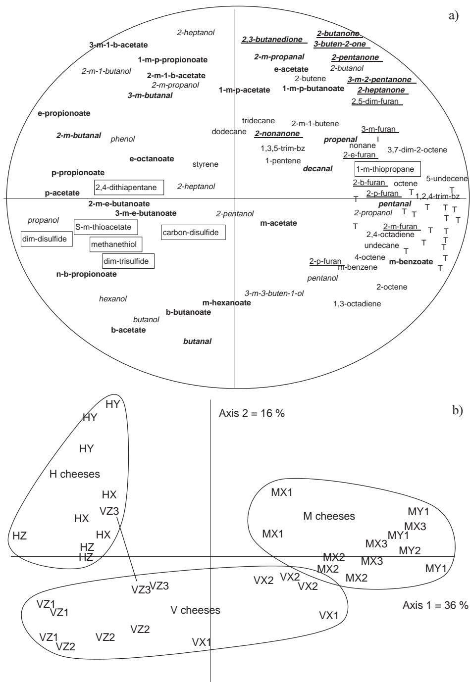
Figure 2. Principal component analysis of the volatile compounds of the cheeses: plot of principal axes 1 and 2.
