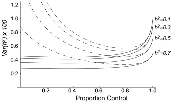
Figure 1. Variance of the maximum likelihood estimator of heritability as a function of the proportion of animals allocated to the control line for the design scheme SC_1 . Full line: model 1 . Dashed line: model 2 .
