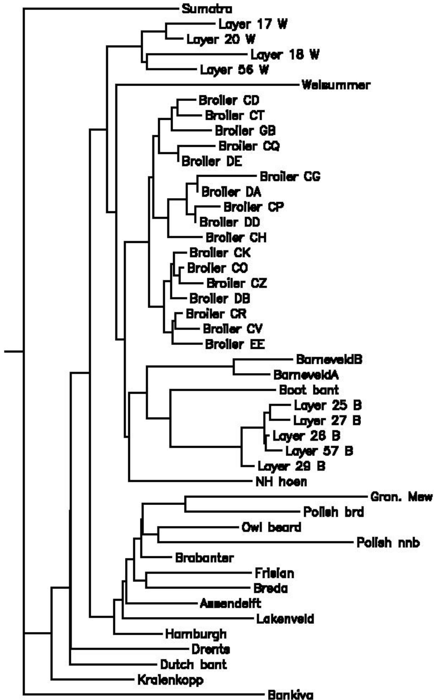
Figure 2. Neighbour-Joining tree representation of relationships between 46 populations of poultry.
