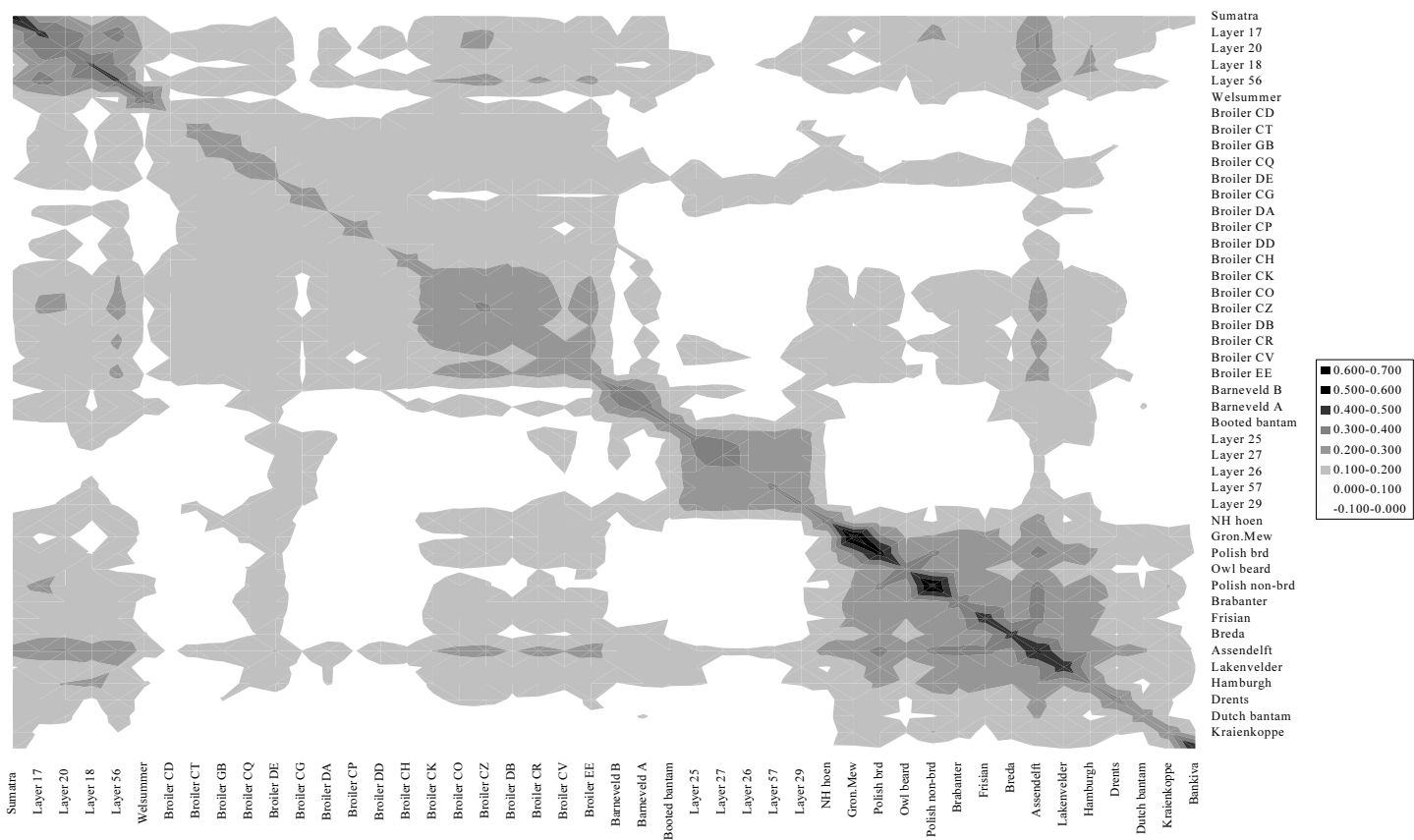
Figure 1. Graphical representation of marker estimated kinship matrix. Shading is dependent on the value of the MEK, where darker shades reflect a higher kinship estimate.
