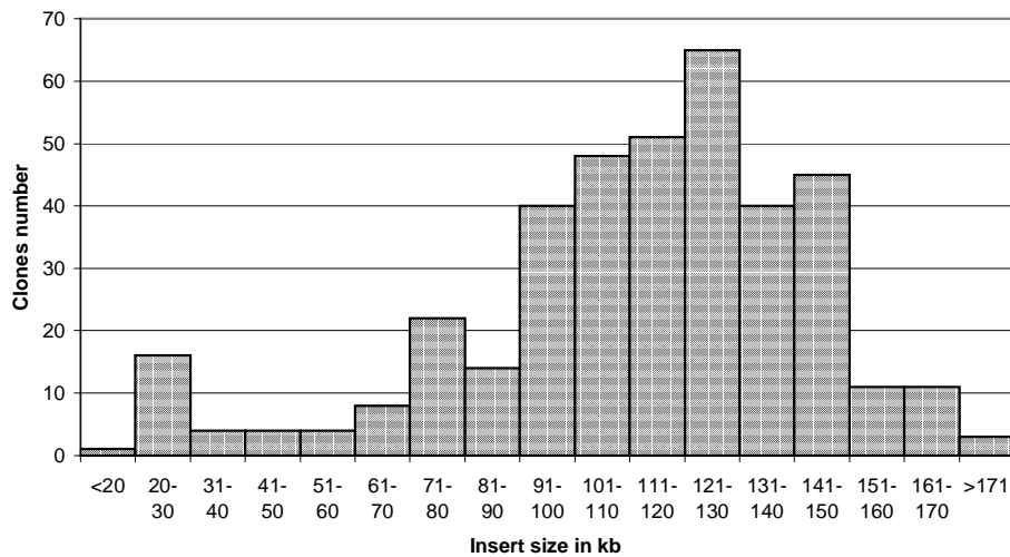
Figure 1. Distribution of insert sizes in the bovine BAC library for a total of 388 clones analysed.
