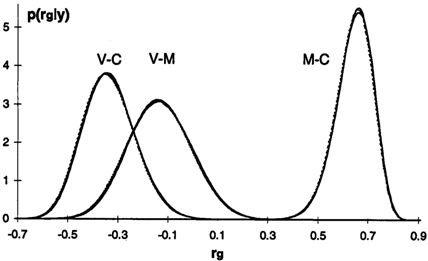
Fig 2. Marginal posterior densities of genetic correlations between the three traits volume (V), motility (M) and concentration (C) obtained with Gibbs sampling (—), Laplace (- - -) or LaplaceE (···) approximation.
