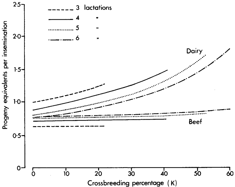
FIG. 2. — Discounted dairy and beef progeny equivalents for varying lactations per cow and percent beef crossing
