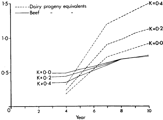
FIG. 1. — Cumulative numbers of discounted beef and dairy progeny equivalents following one insemination in year 0. Four lactations per cow and 85 p. 100 net reproduction are assumed.
