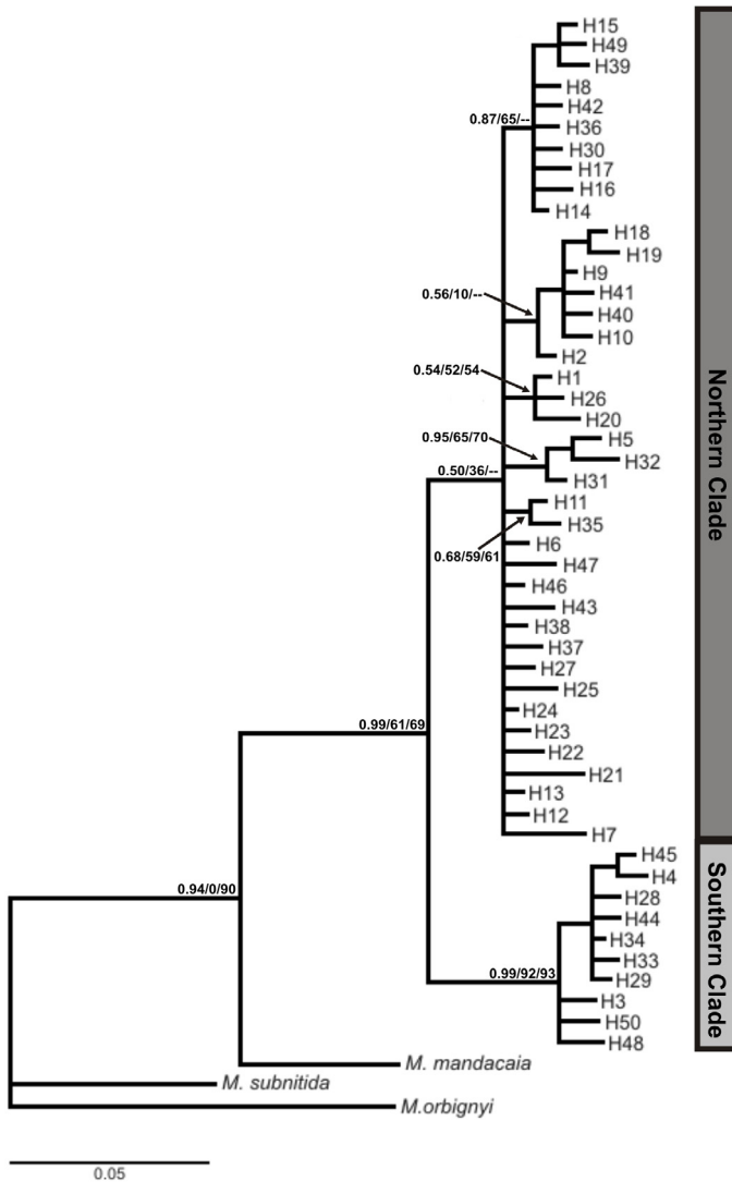
Figure 2. Bayesian inference using the GTR + I model for the COI gene in M. quadrifasciata and outgroups. The haplotypes codes are according to those from Table S1 available in online material. The branch support is expressed as a posteriori Bayesian probabilities and bootstrap values for neighbor-joining and maximum likelihood, respectively.
