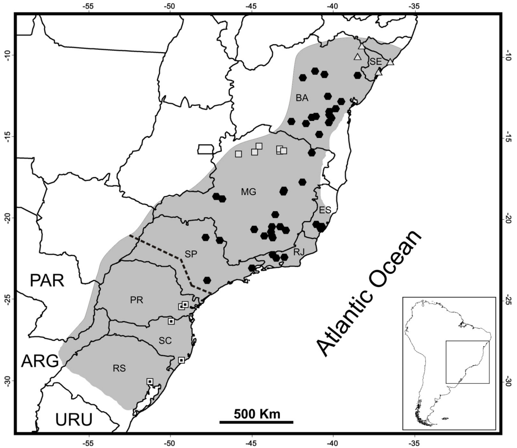
Figure 1. Map of the geographic distribution of the 56 sampling sites of M. quadrifasciata . The white squares with black points indicate individuals of M. q. quadrifasciata , the black hexagons indicate individuals of M. q. anthidioides , the white squares indicate the individuals with continuous tergal stripes from northern Minas Gerais, and the white triangles indicate the specimens with continuous tergal stripes from Sergipe and northeastern Bahia. The grey area represents the geographical range of M. quadrifasciata as determined by Batalha-Filho et al. (2009). The dashed line represents the putative barrier to gene flow estimated with the software SAMOVA 1.0.
