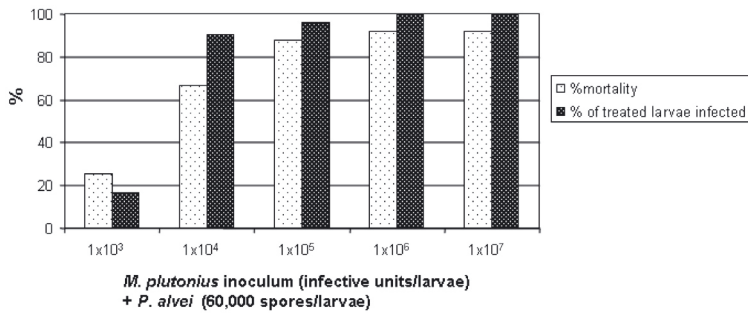
Figure 2. Mortality of honey bee larvae at different infection levels of M. plutonius and secondary infection with P. alvei .
