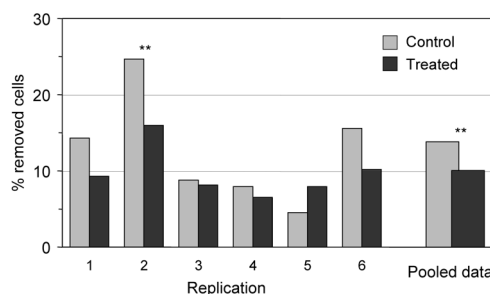
Figure 2. Experiment 1: Proportion of cells emptied by bees in control and treated groups, for each replication and on pooled data. The asterisks indicate significant differences (**: P < 0.01 ).
