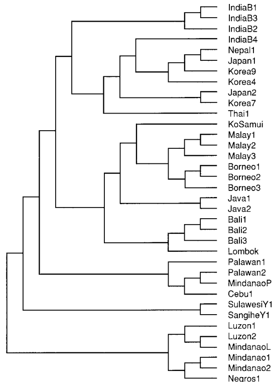
Figure 4. Neighbor-joining tree based on the sequences of 36 non-coding intergenic regions in the mtDNA of A. cerana and A. nigrocincta . Haplotype/sequence names are as in Figure 3 and in Smith and Hagen [23].
