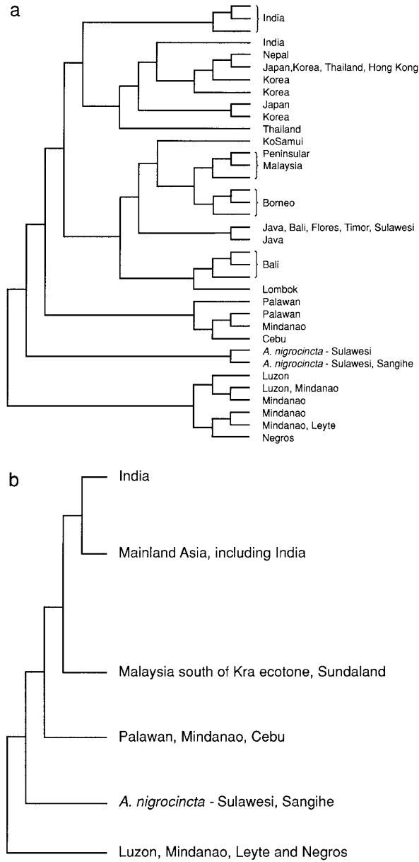
Figure 6. a: Neighbor-joining tree (from Fig. 4) showing the locations in which each haplotype was found. b: Main branches of neighbor-joining tree of A. cerana haplotypes and the geographic region to which each branch corresponds.
