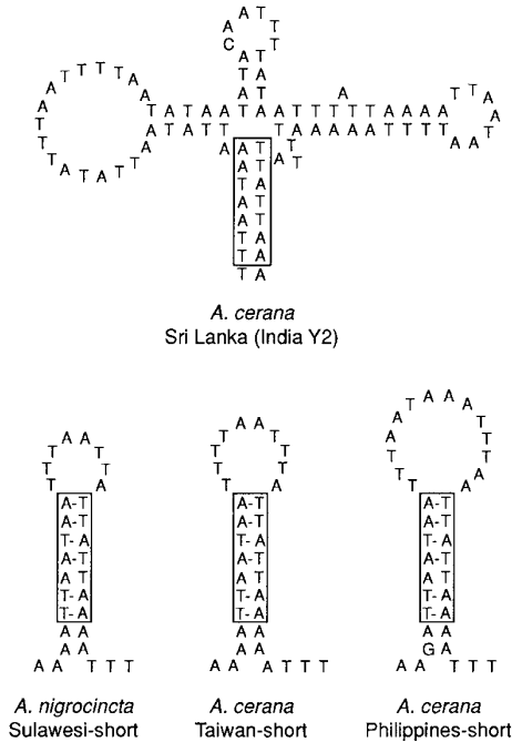
Figure 7. The non-coding sequence of Sri Lankan A. cerana , and the three short sequences: A. cerana TaiwanShort and PhilippineShort, and A. nigrocincta SulawesiShort, showing how they can be folded into clover-leaf and hairpin structures. The clover-leaf structure of Sri Lankan A. cerana is redrawn from Cornuet et al. [1].
