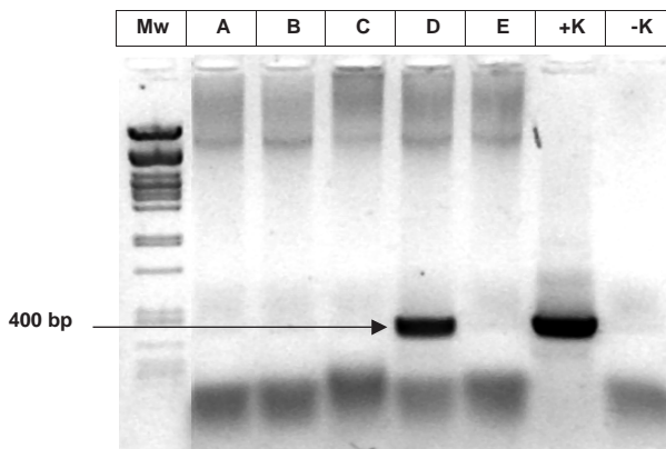
Figure 1. Diagnostic RT-PCR in agarose gel electrophoresis. Mw standard ( PstI cleaved \lambda -phage DNA), A, B, C, E: negative field samples; D: positive field sample, +K: positive control (ABPV inoculated into pupae), -K: negative control.
