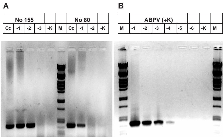
Figure 2. RT-PCR titration A: positive field samples: No. 155 (strong positivity) No. 80 (lower positivity), B: positive control: ABPV inoculated into pupae, Cc: undiluted homogenate, -1: tenfold dilution, -2: 100 fold dilution, -3: 1000 fold dilution, etc., M: standard ( Pst I cleaved \lambda -phage DNA), -K: negative control.
