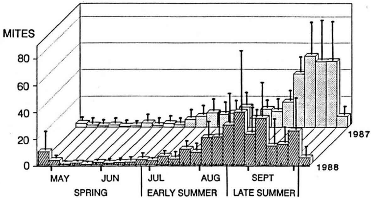
Fig 1. Numbers of Varroa mites monitored weekly from April to October during 1987 and 1988. Abscissa : time of year. Ordinate : means and standard deviations from all monitor colonies, 1987: n = 6 ; 1988: n = 10 .
