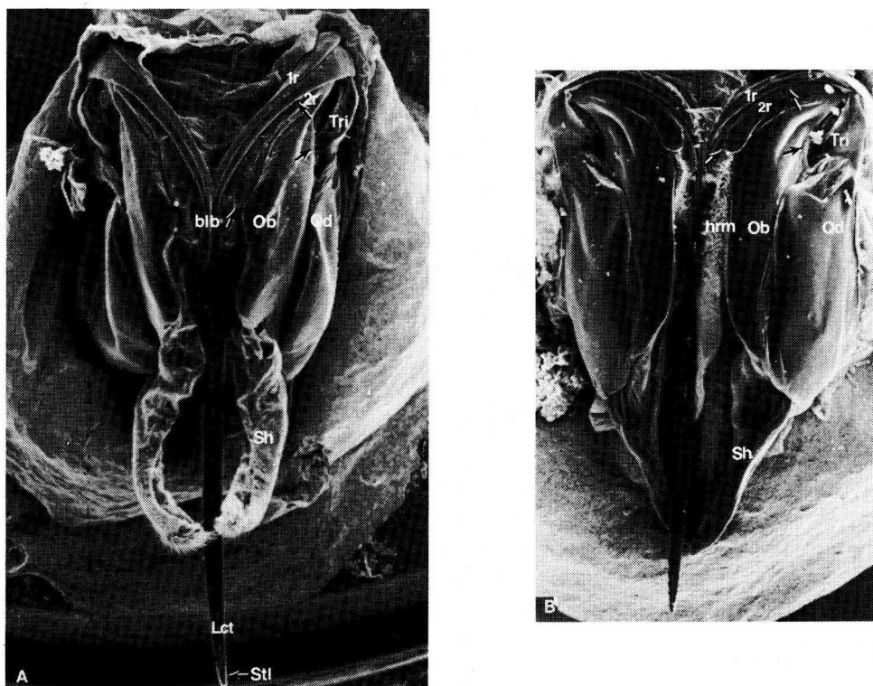
FIG. 1 A. — The sting apparatus of a queen, ventral ( \times 50 ).
