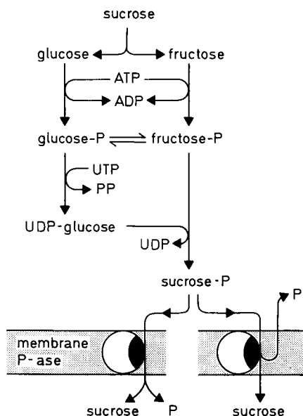
FIG. 2. — Schemes of sucrose transport across a membrane mediated by a membrane phosphatase catalysing « vectorial group transfer ».
